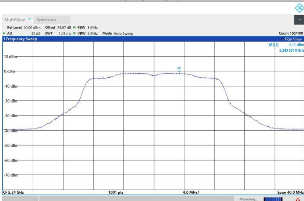
11N20MIMO-Ant2-5240-PASS
