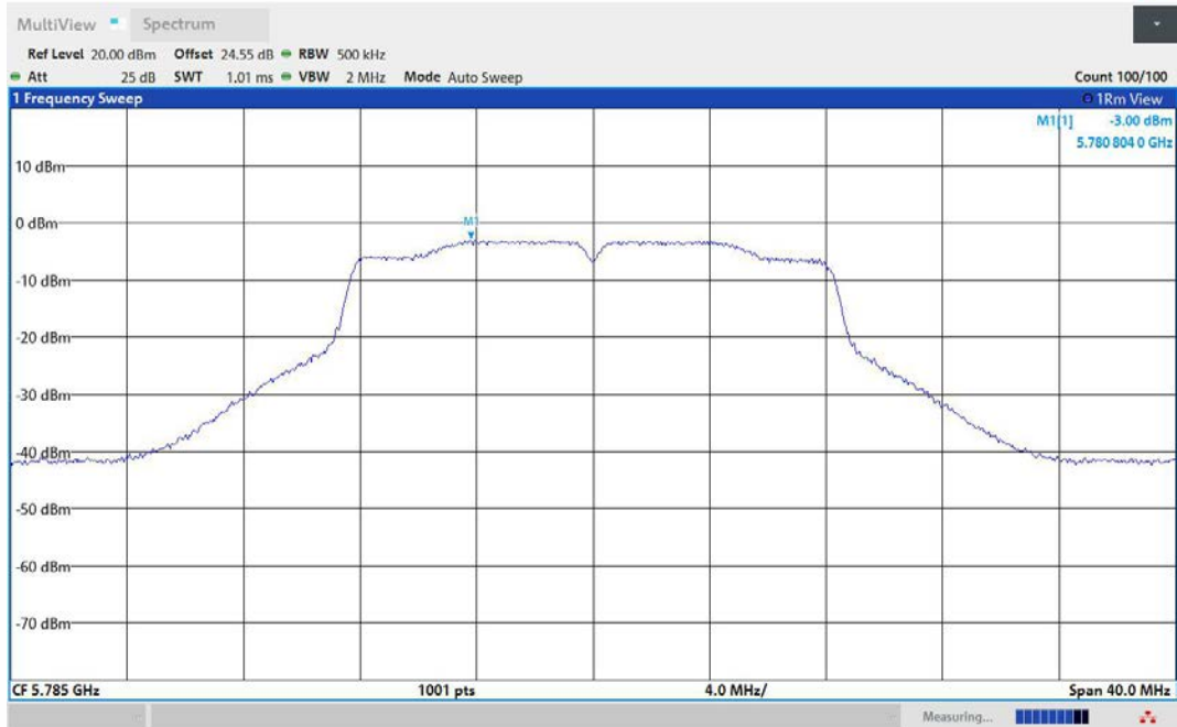
11A-Ant2-5785-PASS
