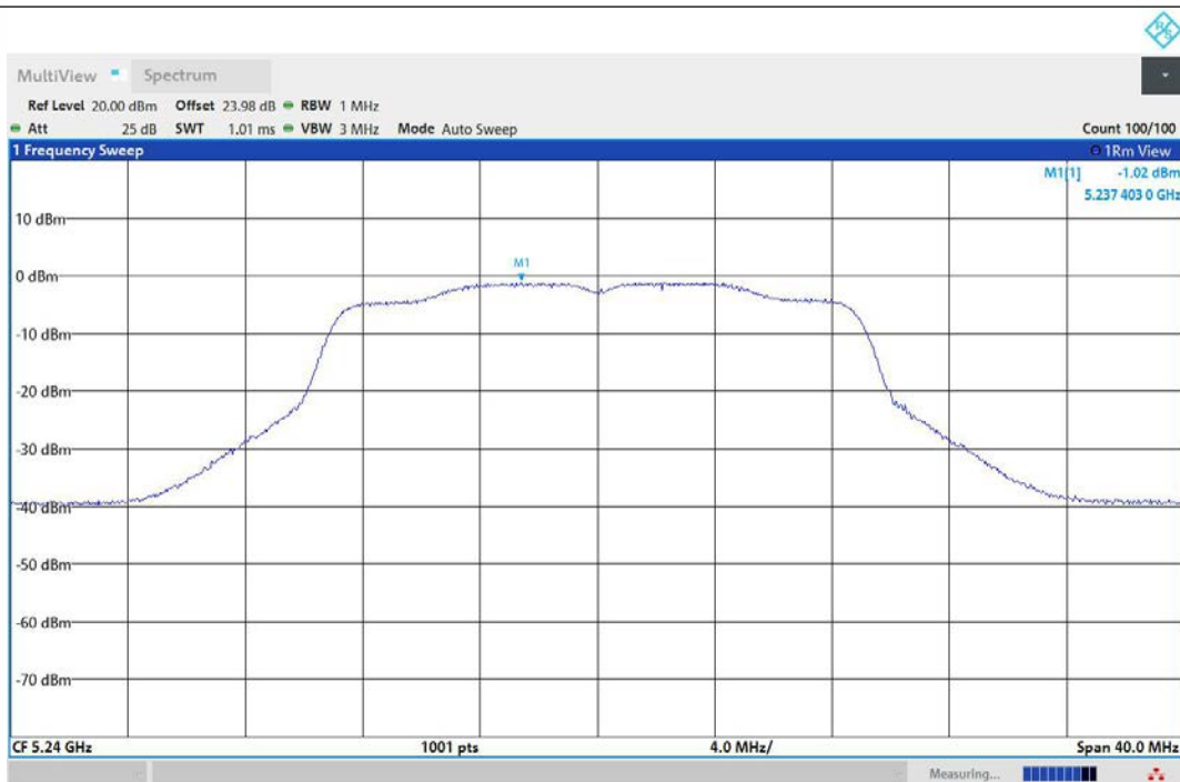
11N20MIMO-Ant1-5240-PASS
