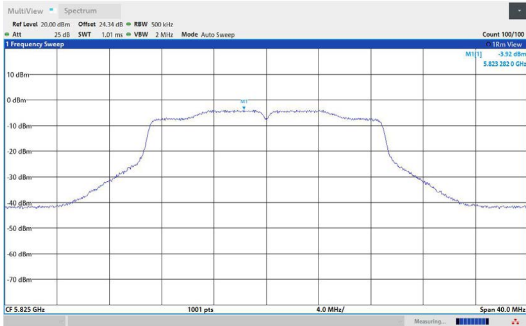
11AC20MIMO-Ant2-5825-PASS
