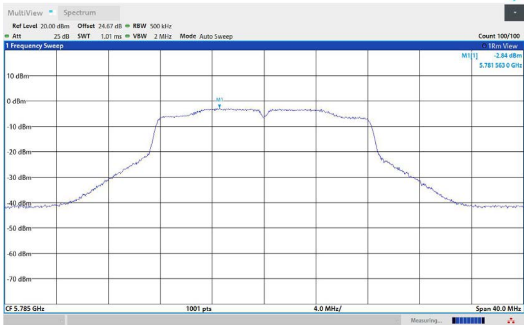
11A-Ant1-5785-PASS
