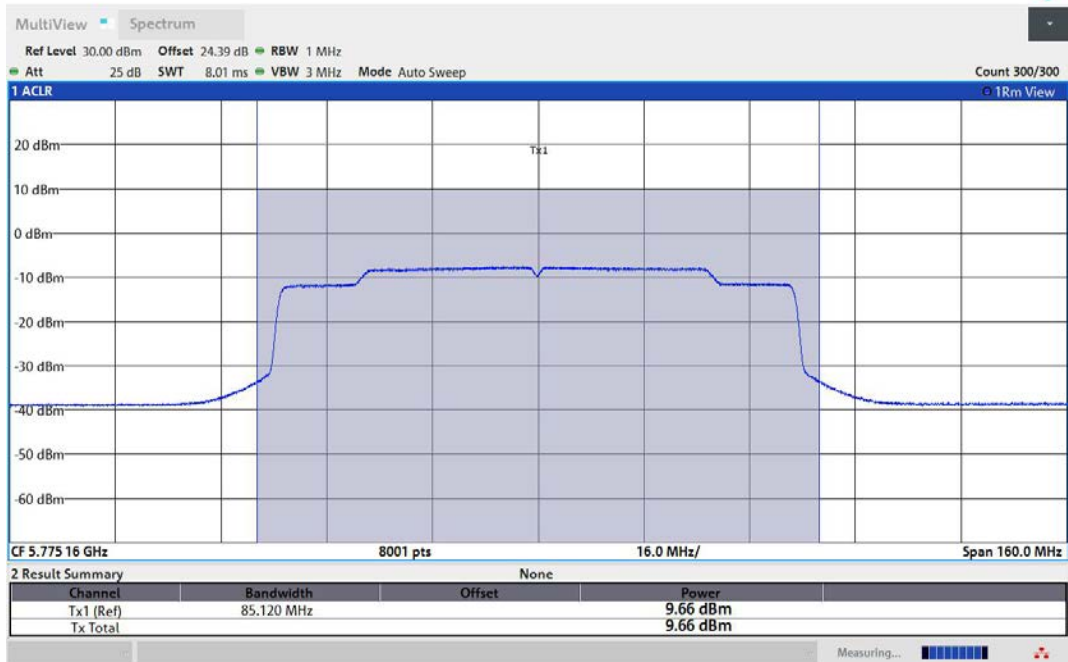
11AX80MIMO-Ant2-5775-PASS
