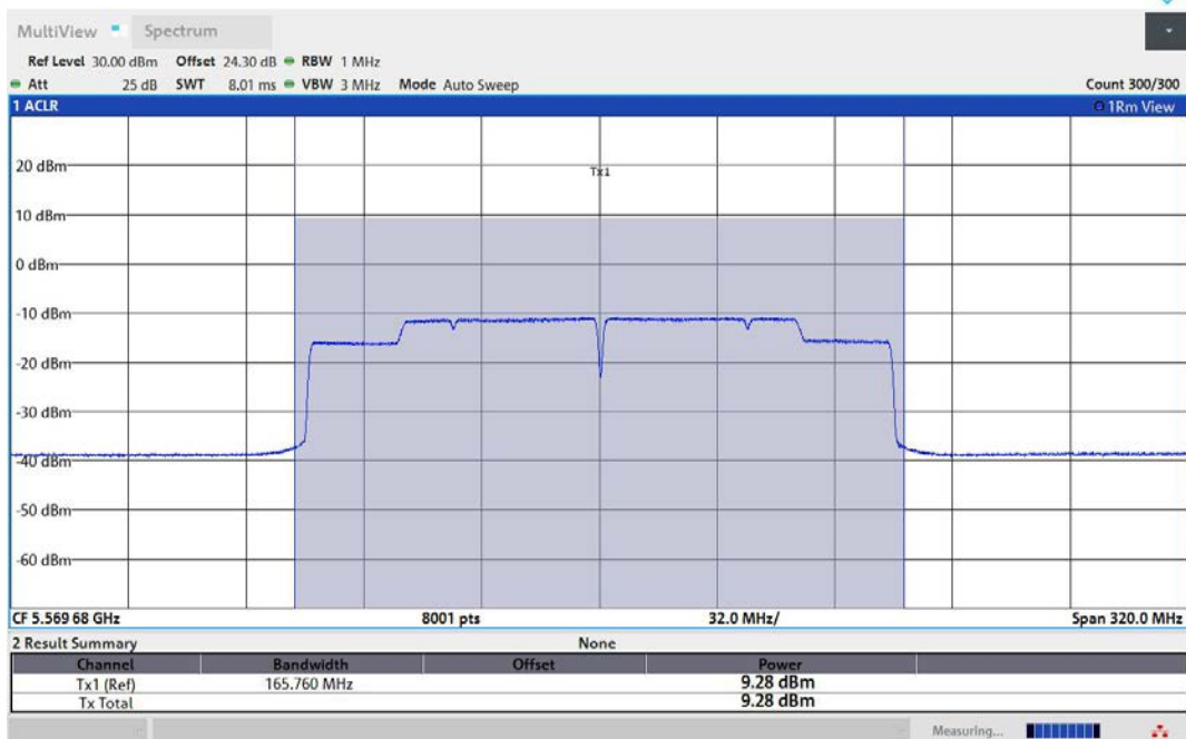
11AX160MIMO-Ant1-5570-PASS
