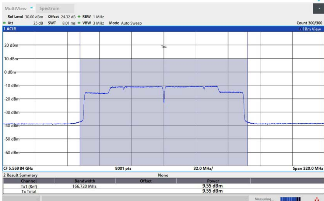
11AX160MIMO-Ant2-5570-PASS
