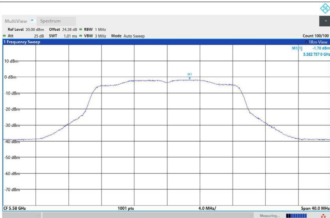
11N20MIMO-Ant1-5580-PASS
