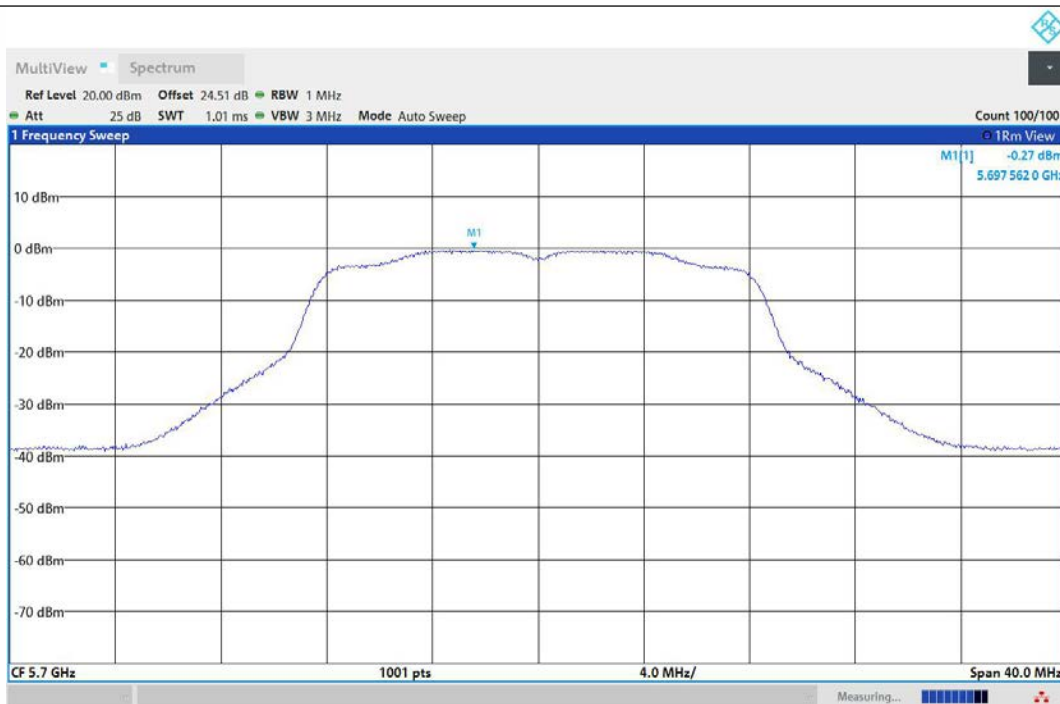
11A-Ant1-5700-PASS
