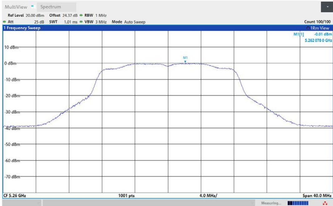
11A-Ant2-5260-PASS
