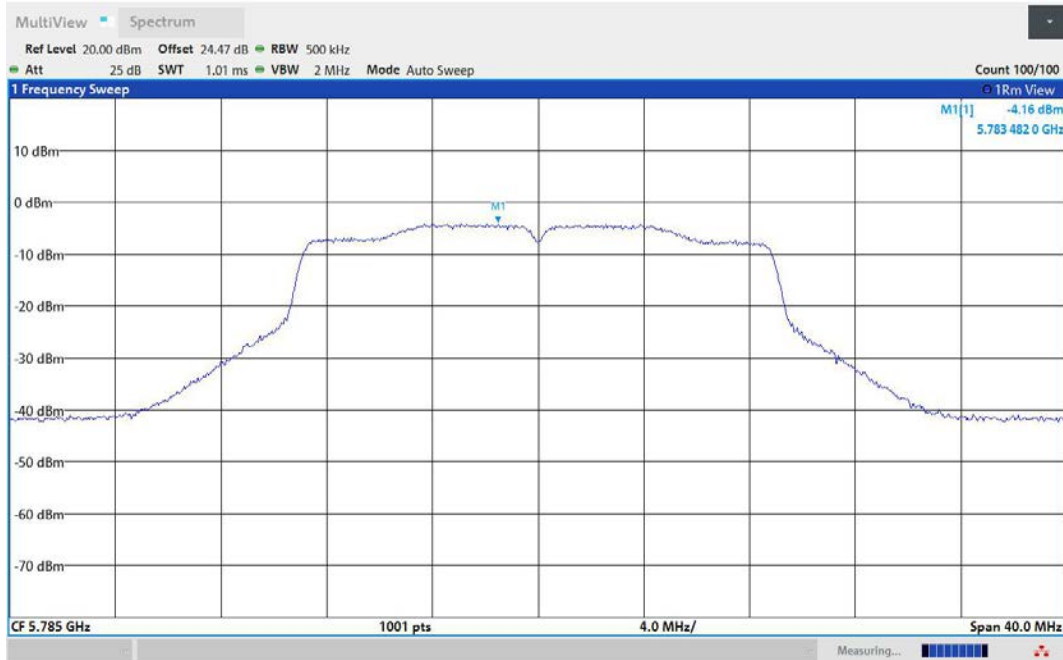
11AC20MIMO-Ant2-5785-PASS
