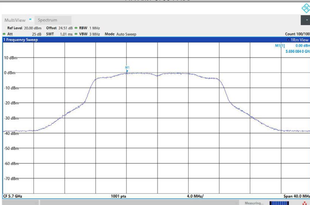
11A-Ant2-5700-PASS
