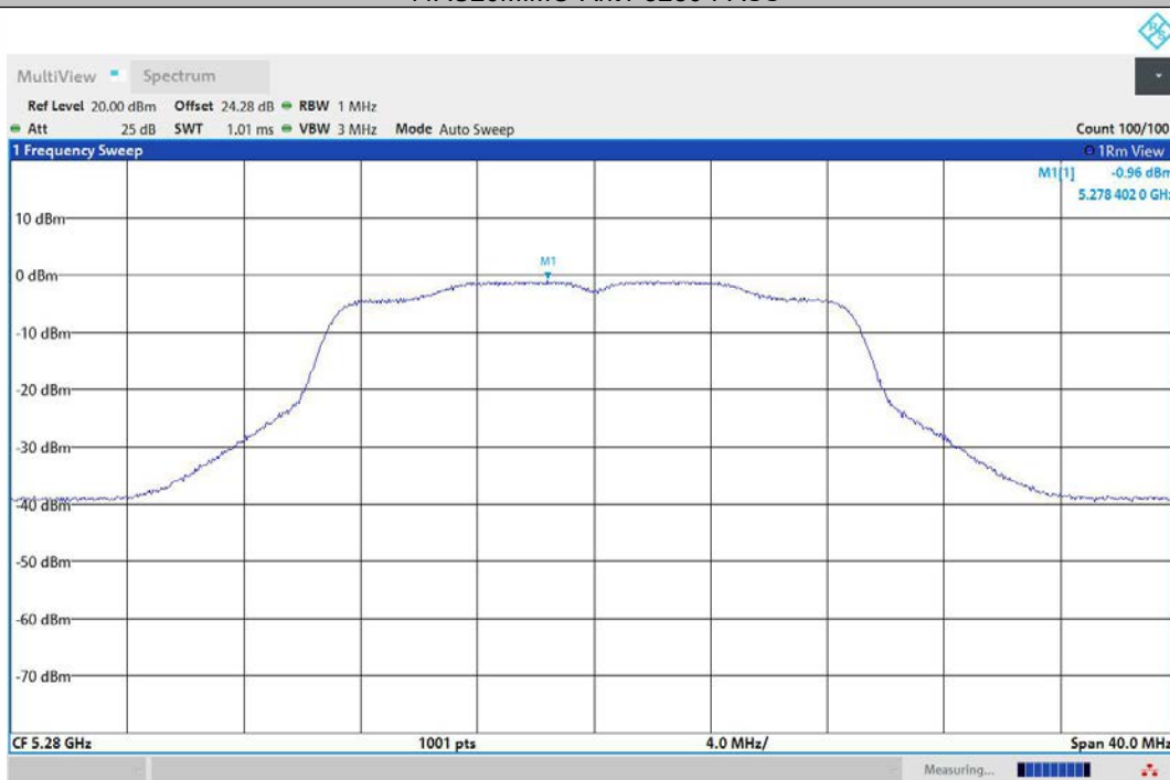
11AC20MIMO-Ant2-5280-PASS
