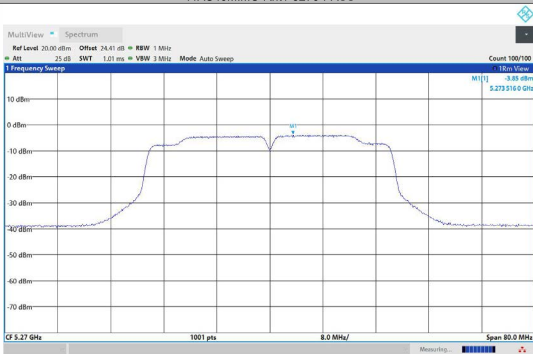
11AC40MIMO-Ant2-5270-PASS
