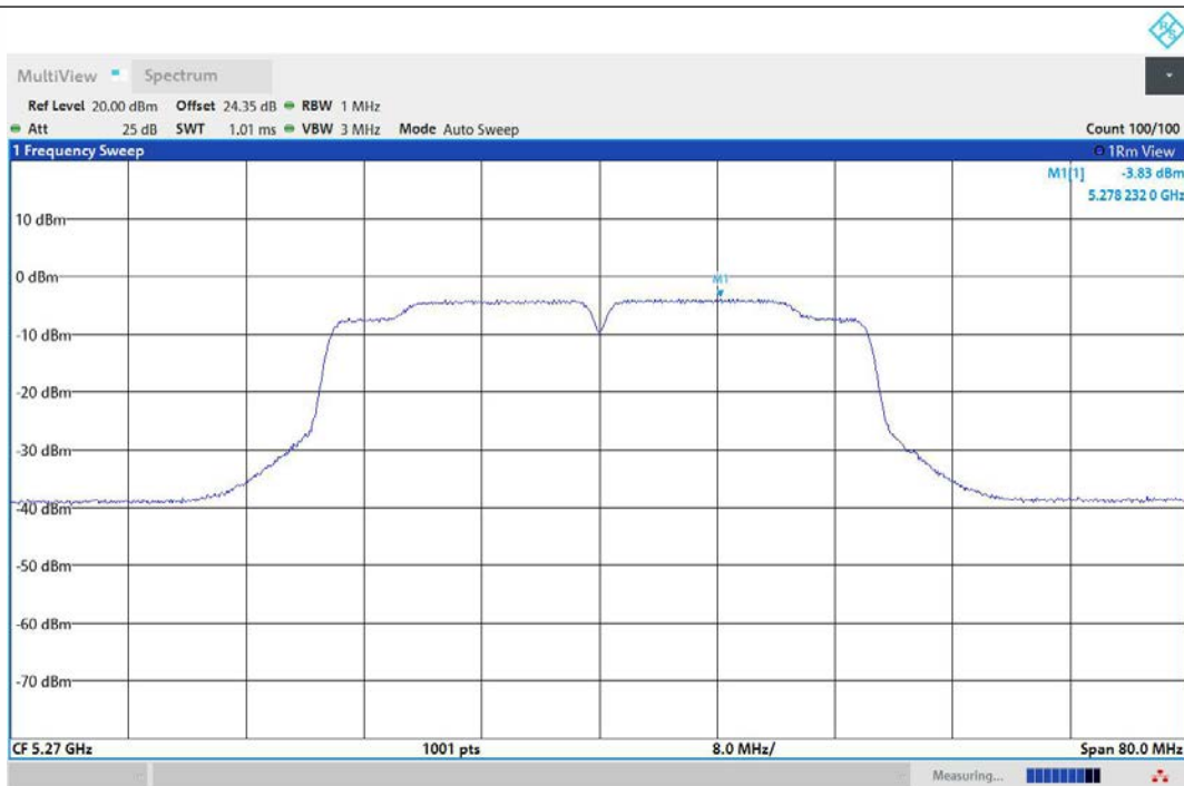
11AC40MIMO-Ant1-5270-PASS
