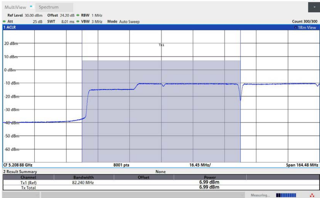
11AX160MIMO-Ant2-5250_UNII-1-PASS
