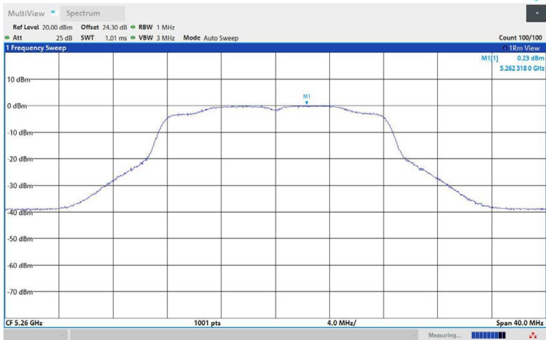
11A-Ant1-5260-PASS
