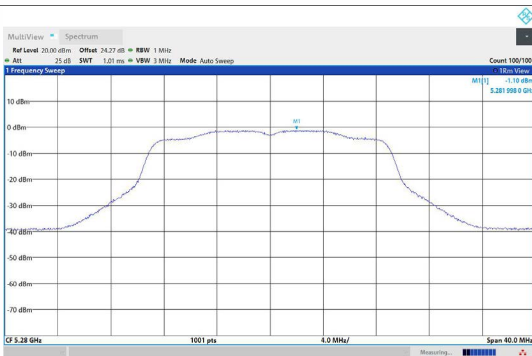
11AC20MIMO-Ant1-5280-PASS
