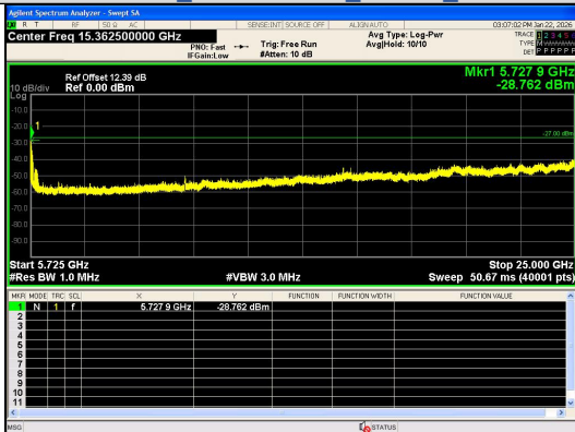
Spurious Emission:5725~25000.0 MHz IEEE 802.11ac_Channel 120_20MHz_Antenna 0
