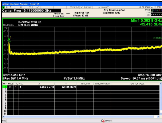
Spurious Emission:5350~25000.0 MHz IEEE 802.11ac_Channel 64_20MHz_Antenna 0
