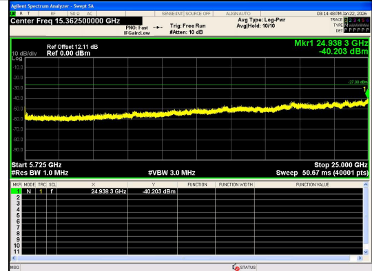
Spurious Emission:5725~25000.0 MHz IEEE 802.11ac_Channel 100_20MHz_Antenna 0
