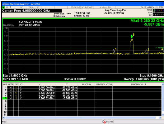
Out Of Band Emission IEEE 802.11ax_Channel 52_20MHz_Antenna 0_RU&Index SU
