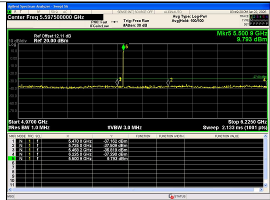
Out Of Band Emission IEEE 802.11ax_Channel 100_20MHz_Antenna 0_RU&Index SU
