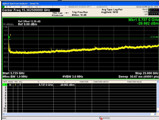
Spurious Emission:5725~25000.0 MHz IEEE 802.11ax_Channel 120_20MHz_Antenna 0_RU&Index SU
