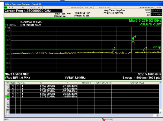
Out Of Band Emission IEEE 802.11ax_Channel 56_20MHz_Antenna 0_RU&Index SU
