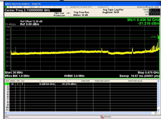
Spurious Emission:30.0~5470 MHz IEEE 802.11ax_Channel 120_20MHz_Antenna 0_RU&Index SU
