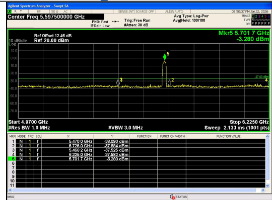
Out Of Band Emission IEEE 802.11ax_Channel 140_20MHz_Antenna 0_RU&Index SU
