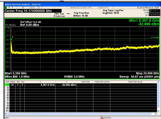
Spurious Emission:5350~25000.0 MHz IEEE 802.11ax_Channel 56_20MHz_Antenna 0_RU&Index SU
