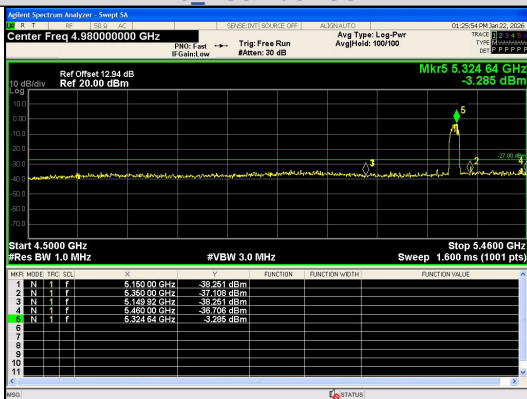
Out Of Band Emission IEEE 802.11ax_Channel 64_20MHz_Antenna 0_RU&Index SU
