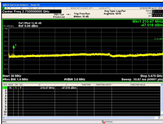
Spurious Emission:30.0~5470 MHz IEEE 802.11ax_Channel 140_20MHz_Antenna 0_RU&Index SU
