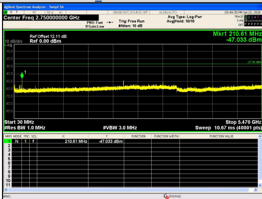
Spurious Emission:30.0~5470 MHz IEEE 802.11ax_Channel 100_20MHz_Antenna 0_RU&Index SU
