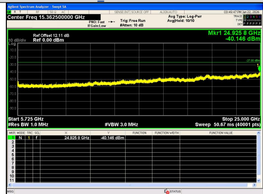
Spurious Emission:5725~25000.0 MHz IEEE 802.11ax_Channel 100_20MHz_Antenna 0_RU&Index SU
