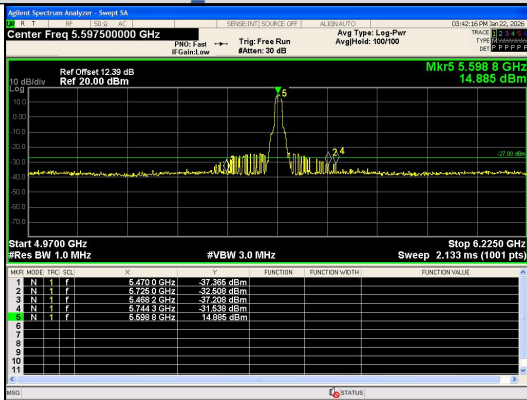
Out Of Band Emission IEEE 802.11ax_Channel 120_20MHz_Antenna 0_RU&Index SU
