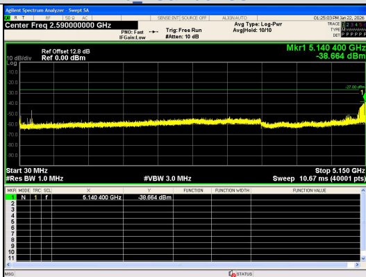
Spurious Emission:30.0~5150 MHz IEEE 802.11ax_Channel 56_20MHz_Antenna 0_RU&Index SU
