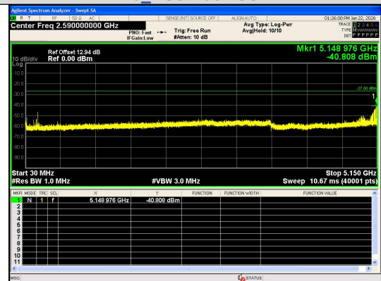
Spurious Emission:30.0~5150 MHz IEEE 802.11ax_Channel 64_20MHz_Antenna 0_RU&Index SU
