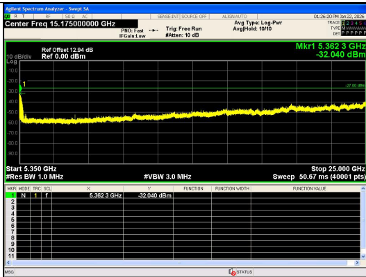
Spurious Emission:5350~25000.0 MHz IEEE 802.11ax_Channel 64_20MHz_Antenna 0_RU&Index SU
