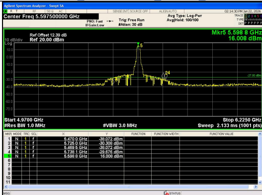
Out Of Band Emission IEEE 802.11n_Channel 120_20MHz_Antenna 0
