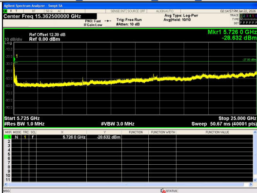
Spurious Emission:5725~25000.0 MHz IEEE 802.11n_Channel 120_20MHz_Antenna 0
