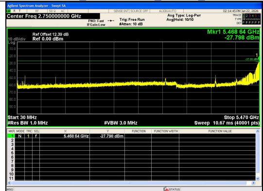
Spurious Emission:30.0~5470 MHz IEEE 802.11n_Channel 120_20MHz_Antenna 0
