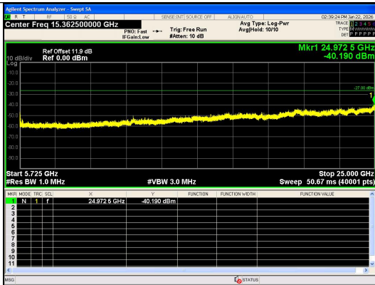
Spurious Emission:5725~25000.0 MHz IEEE 802.11n Channel 102 40MHz Antenna 0
