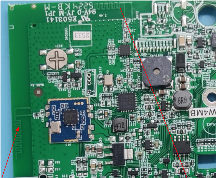
WIFI 2.4G Antenna location
