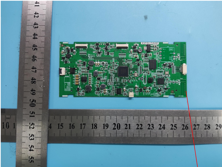
2.4G Antenna location
