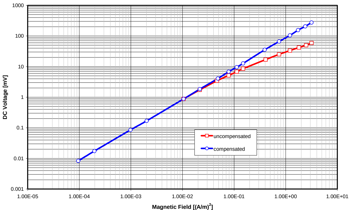
Dynamic Range, Probe S/N 101, 835MHz
