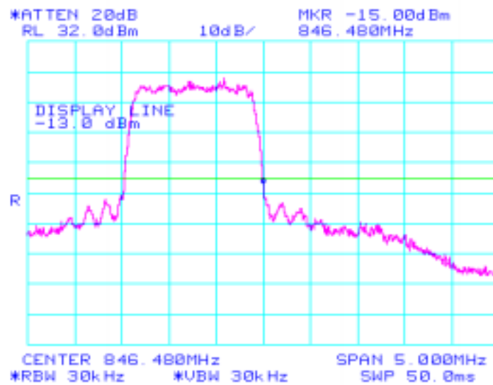
High Channel Bandedge 692
