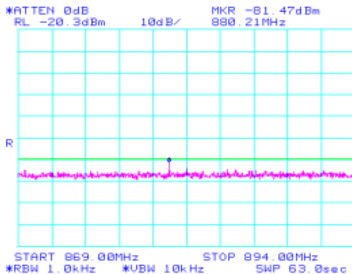
Low Channel Mobile emissions
