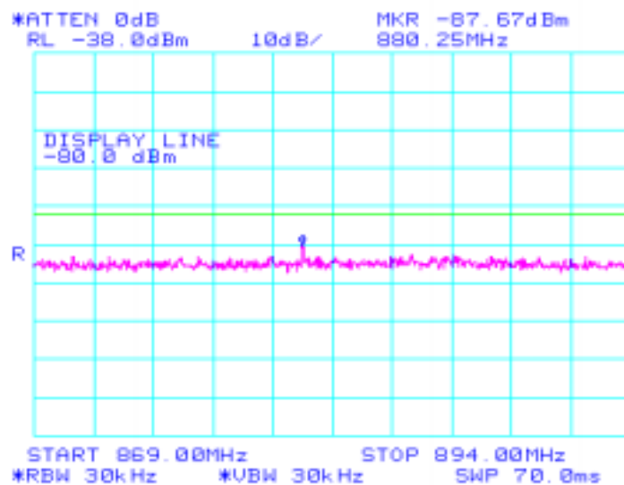
RSS-129 (10)(b) Rx
