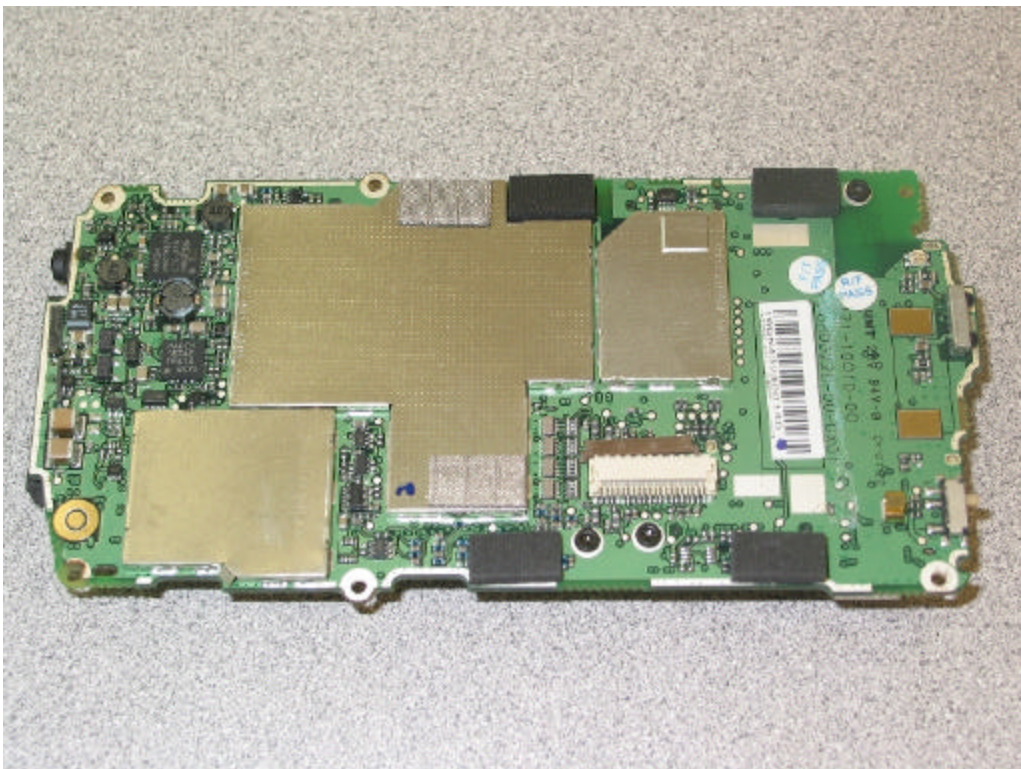
Main PCB w/ foam removed
