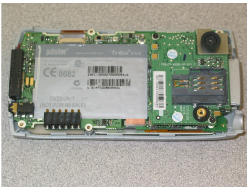
Main PCB w/ RF module installed
