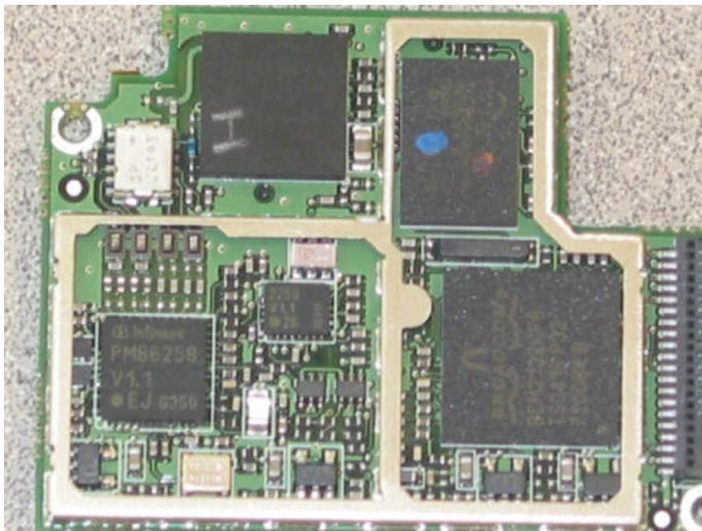
RF Module Detail
