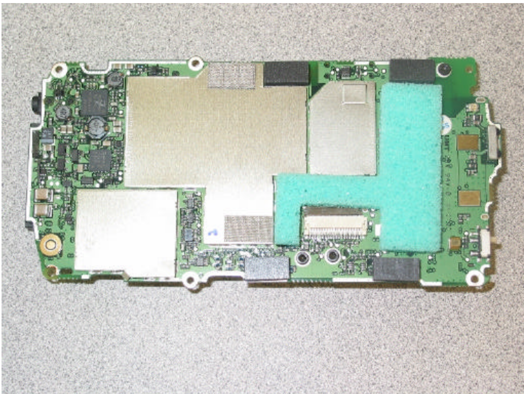
Main PCB detail, w/ shields
