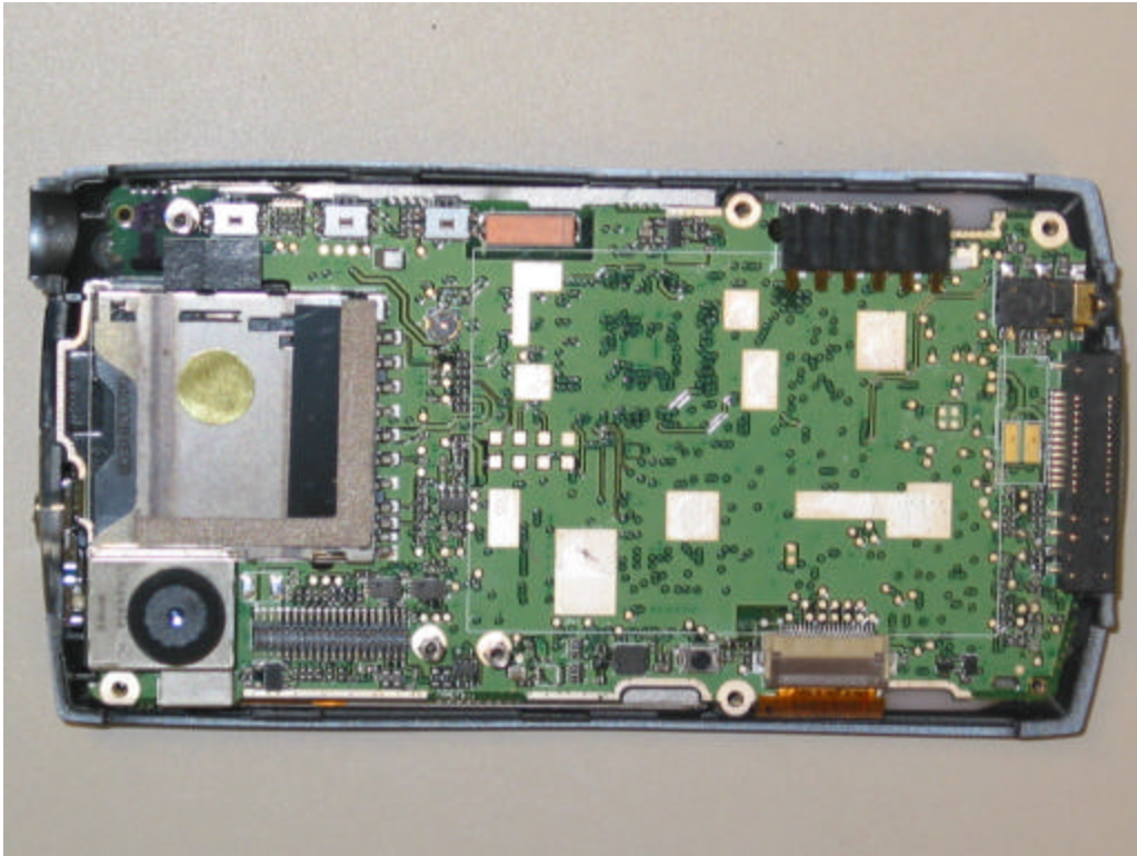
Main PCB with RF module and label removed
