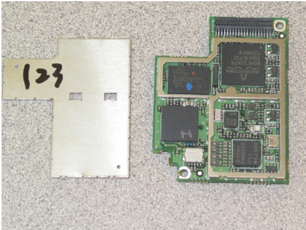
RF Module, Shield Side w/ Shield removed
