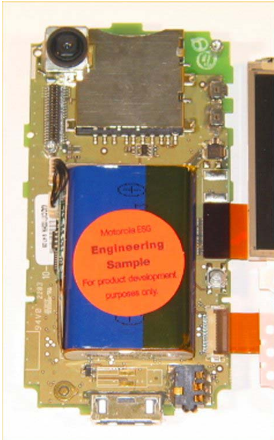
Treo 600 Main PCA, RF module removed.
