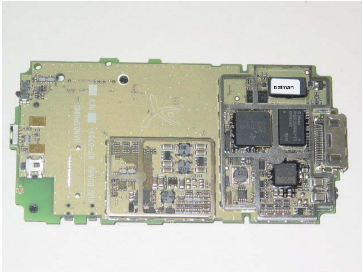
Treo 600 Main PCA, Foam removed
