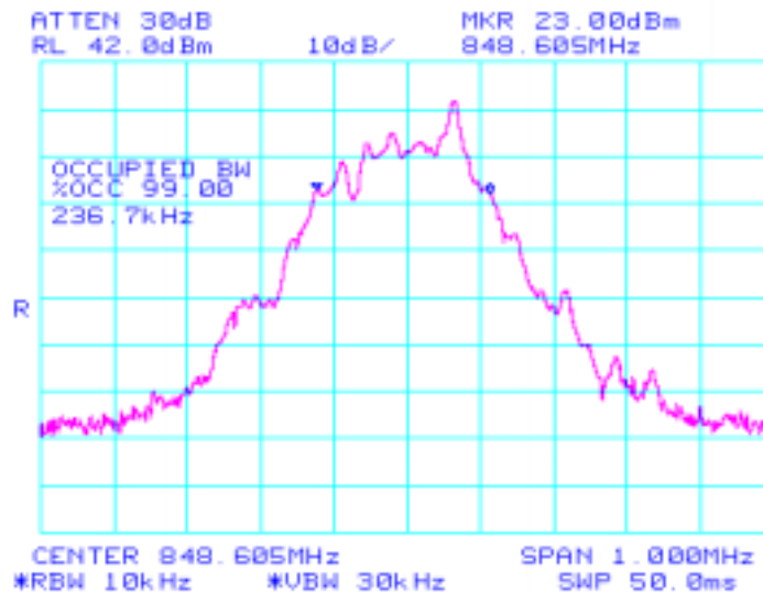
High Channel 99% BW
