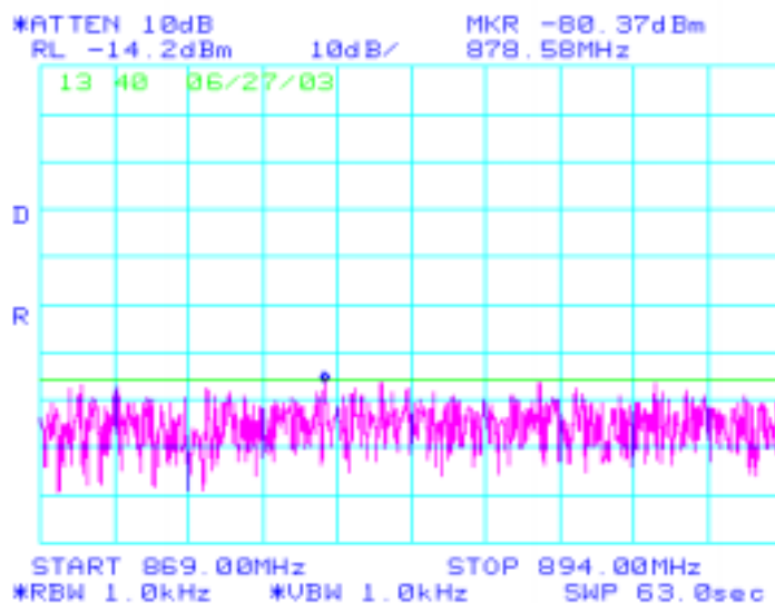
Low Channel Mobile Emission
