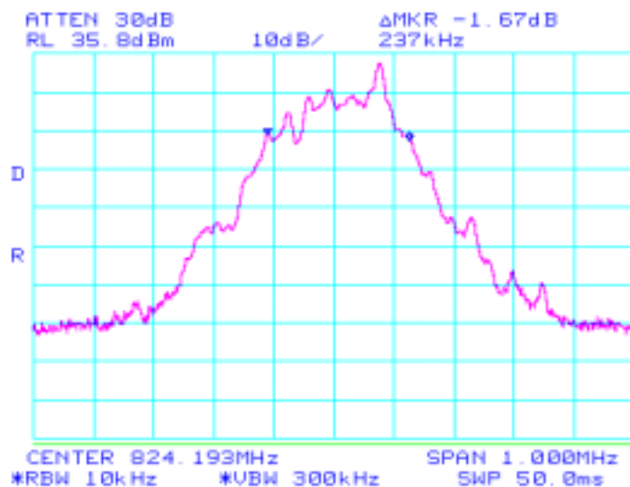
Low Channel 99% Bandwidth
