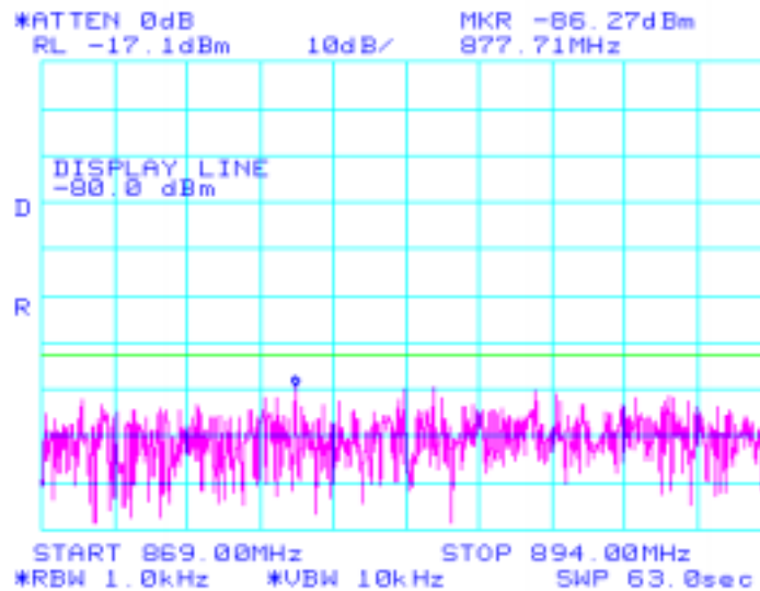
High Channel mobile emissions
