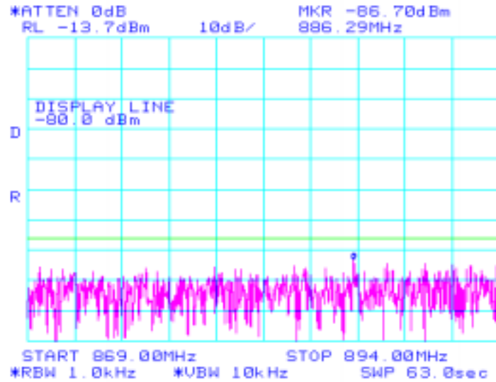
Low Channel Mobile emission
