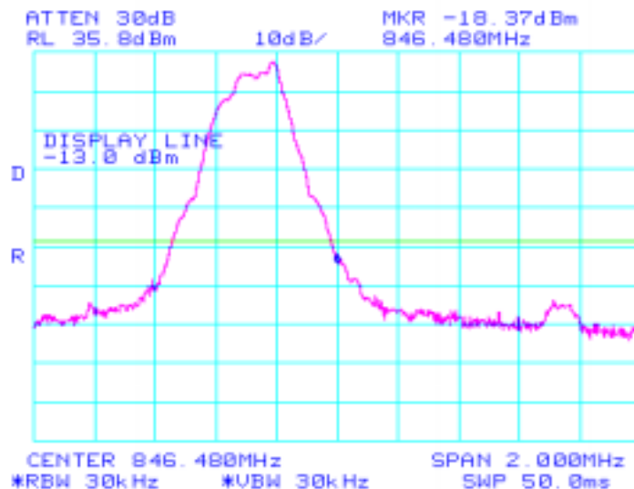
High Block A Bandedge
