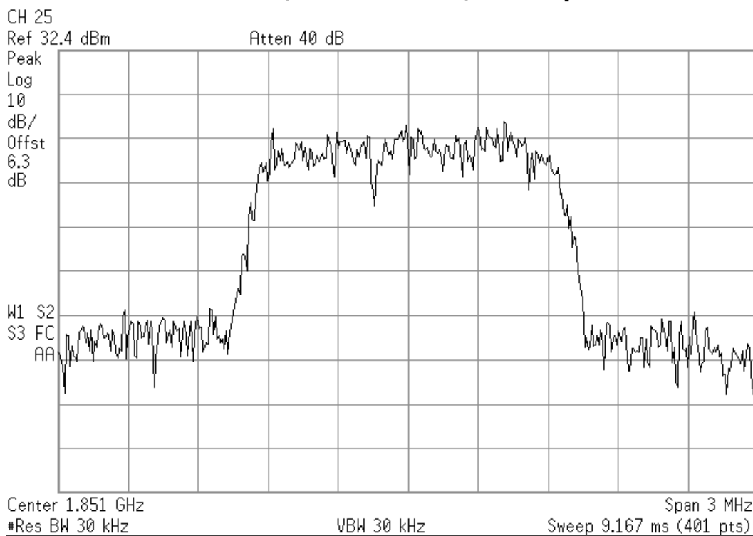
PCS band, low channel, wideband
