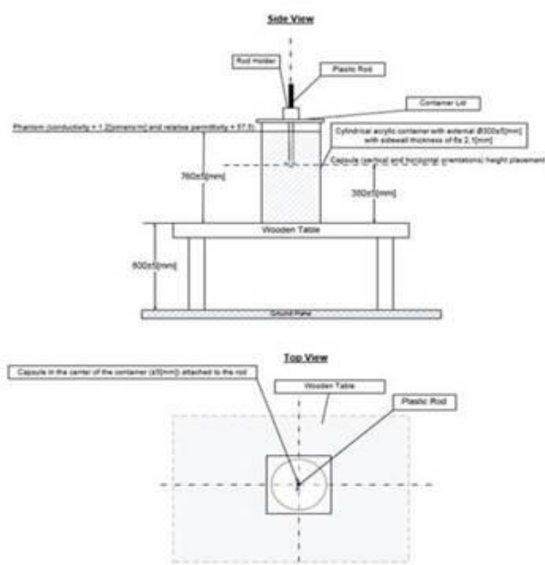
Figure 2: test setup
