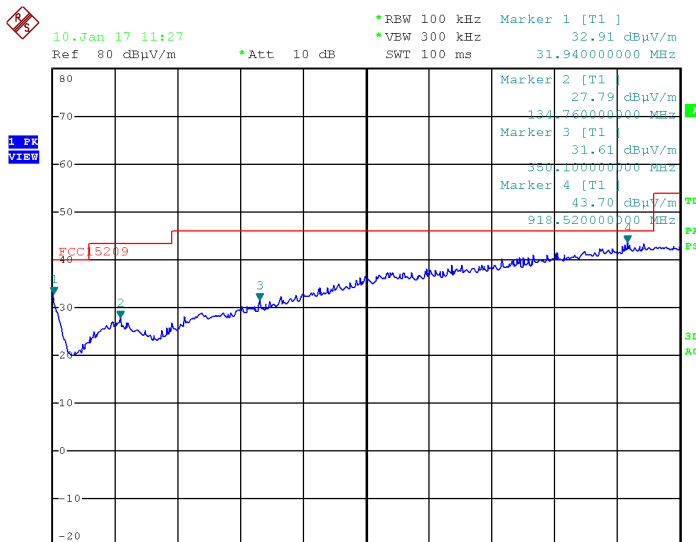
Plot 1a Radiated emissions (Peak values) of the EUT in the frequency range 30 – 1000 MHz, EUT Vertical, Antenna Horizontal
