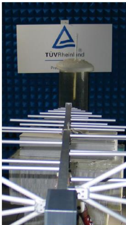
Photograph of the test setup
