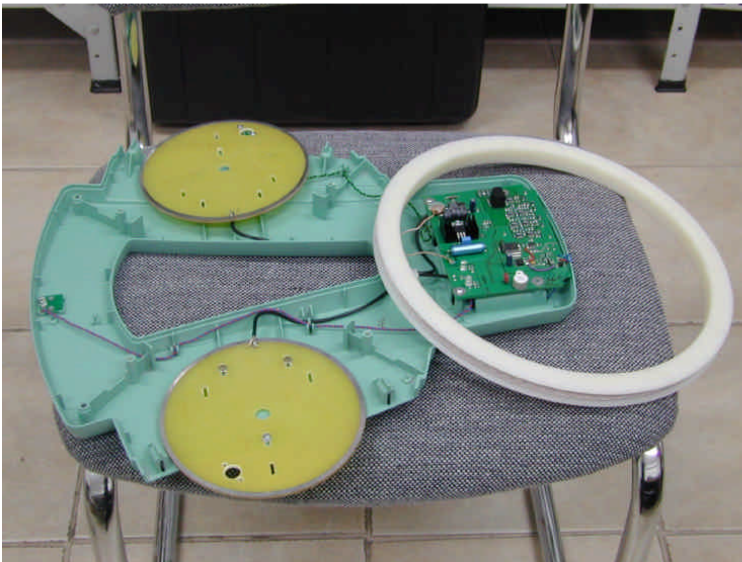
Internal view with exciter antenna removed
