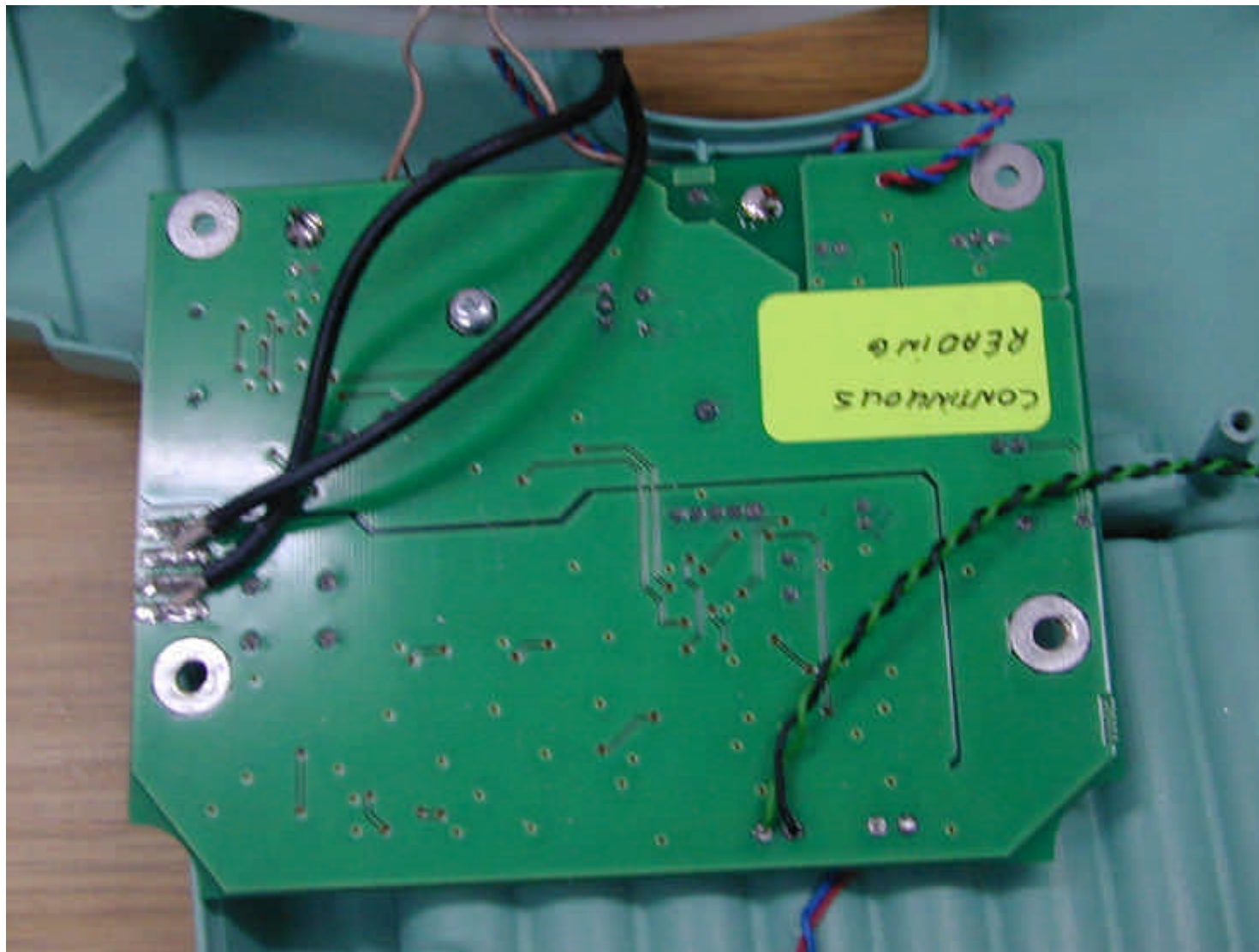
PCB first side
