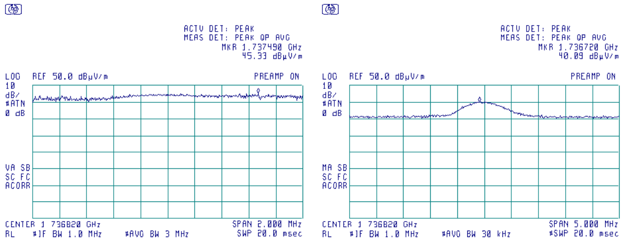
Plot 7.2.16 Radiated emission measurements at the fourth harmonic frequency
