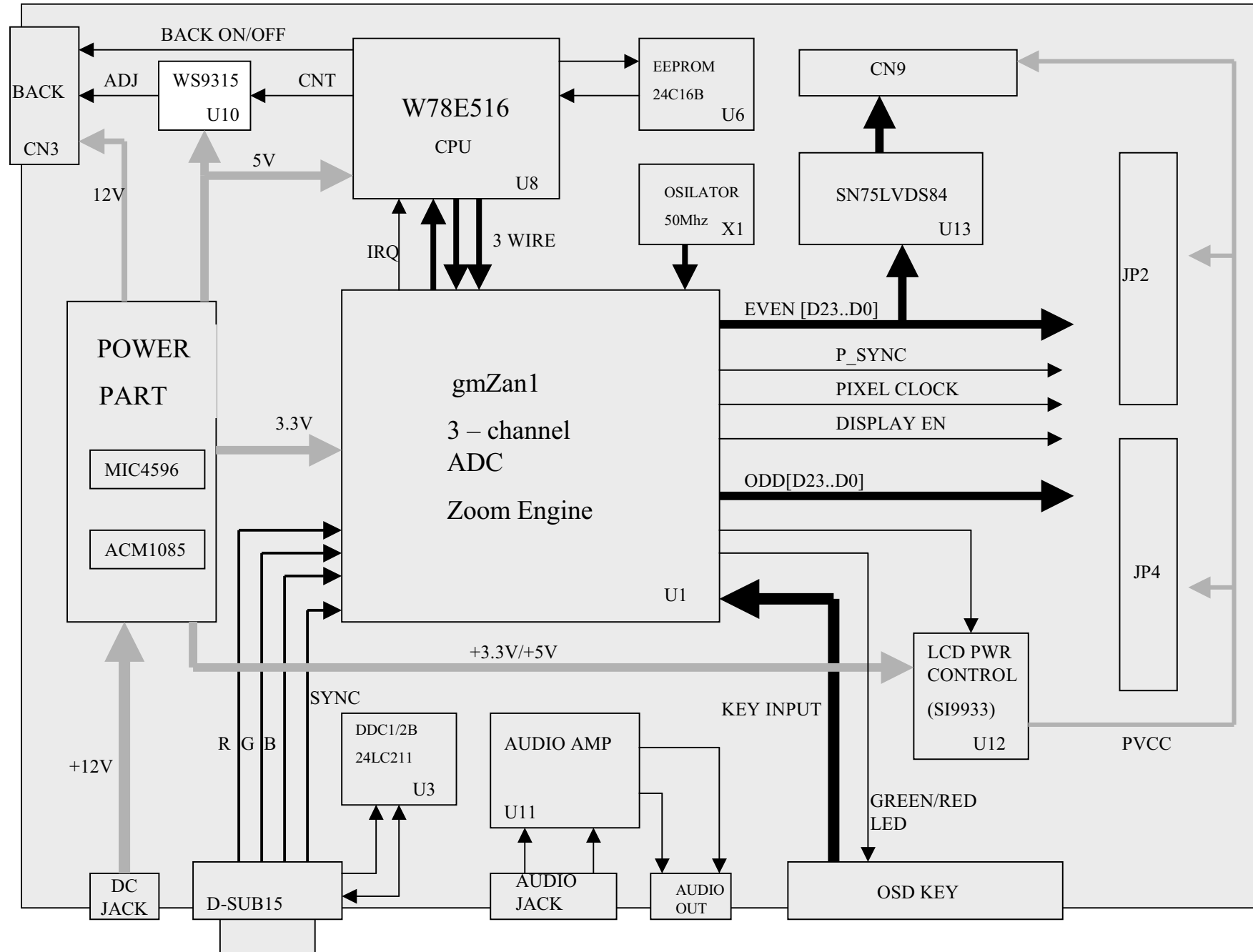
VT-M101 BLOCK DIAGRAM
