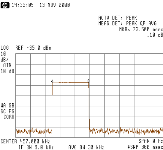
Detail of a previous pulse
