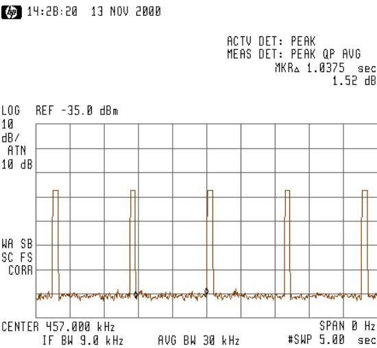
Pulsed signal versus time, for a zero span
