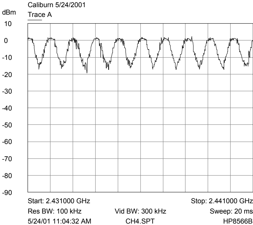
Number of Hopping Channels (Plot 4)
