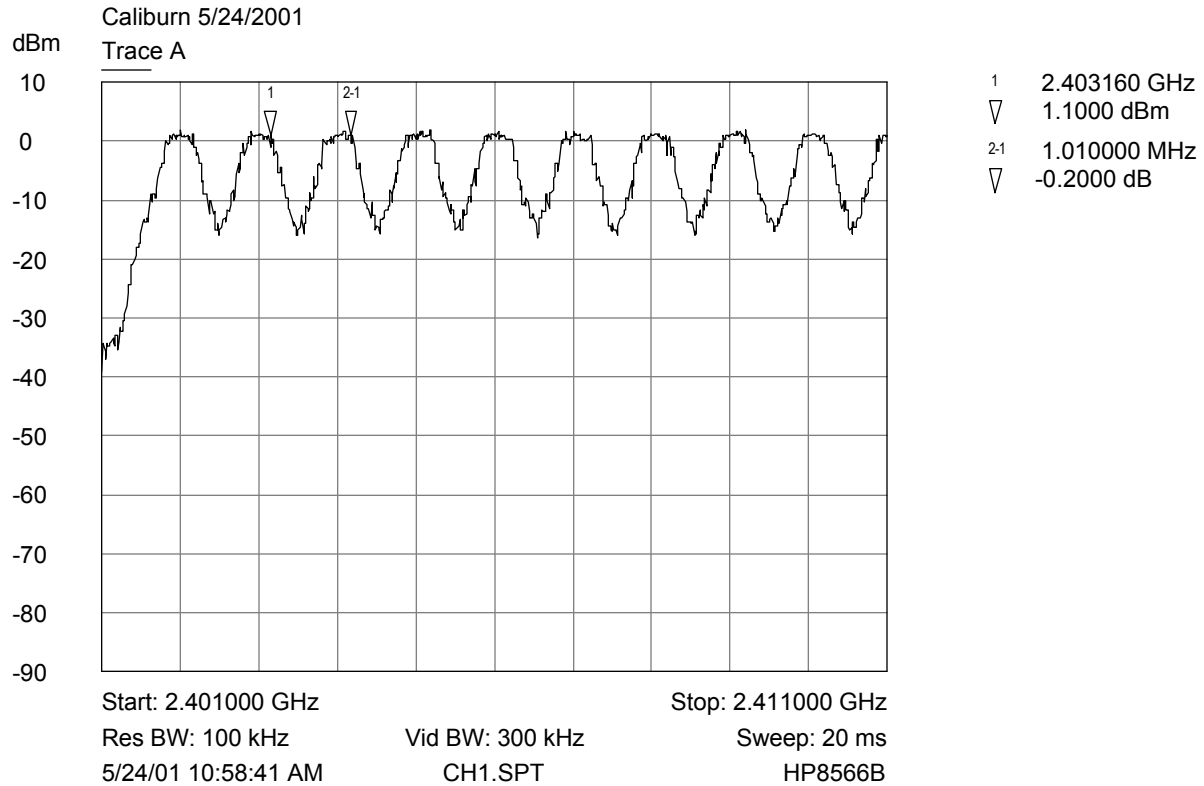
Number of Hopping Channels (Plot 1)
