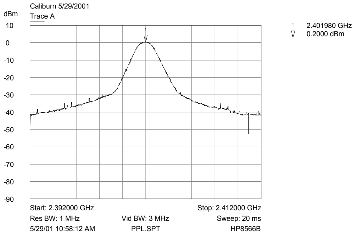
Peak Output Power Plot - (Low Channel)
