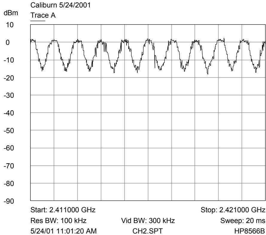
Number of Hopping Channels (Plot 2)
