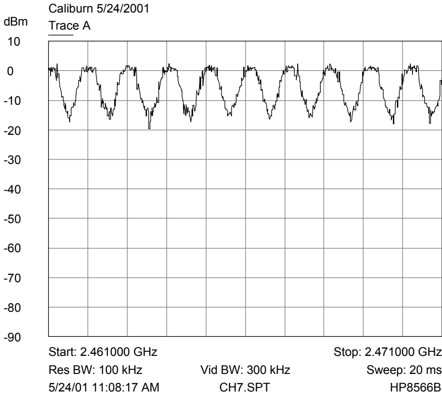
Number of Hopping Channels (Plot 7)
