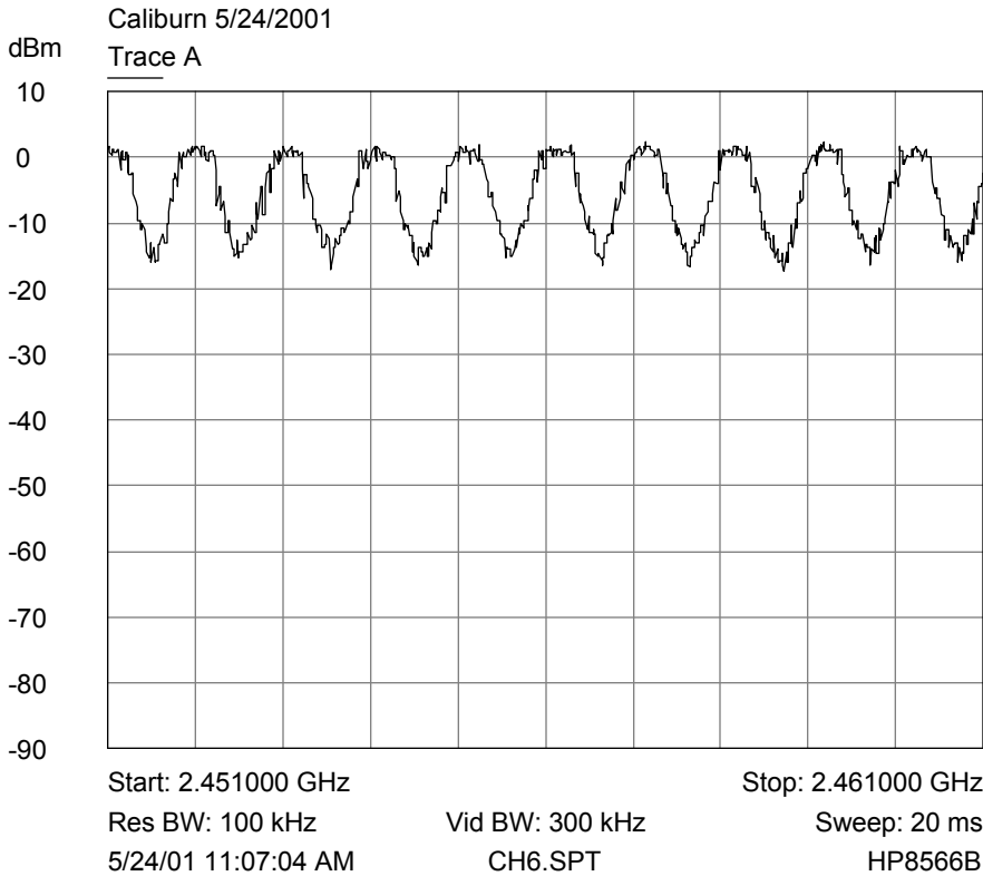
Number of Hopping Channels (Plot 6)
