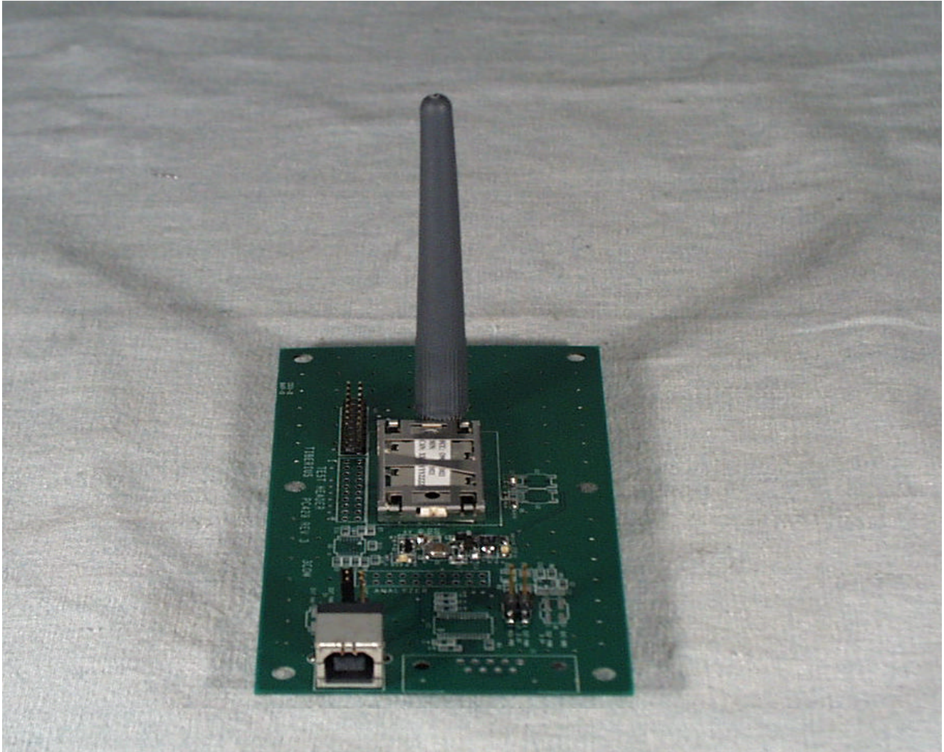
End View of the Tiberius Test Platform
