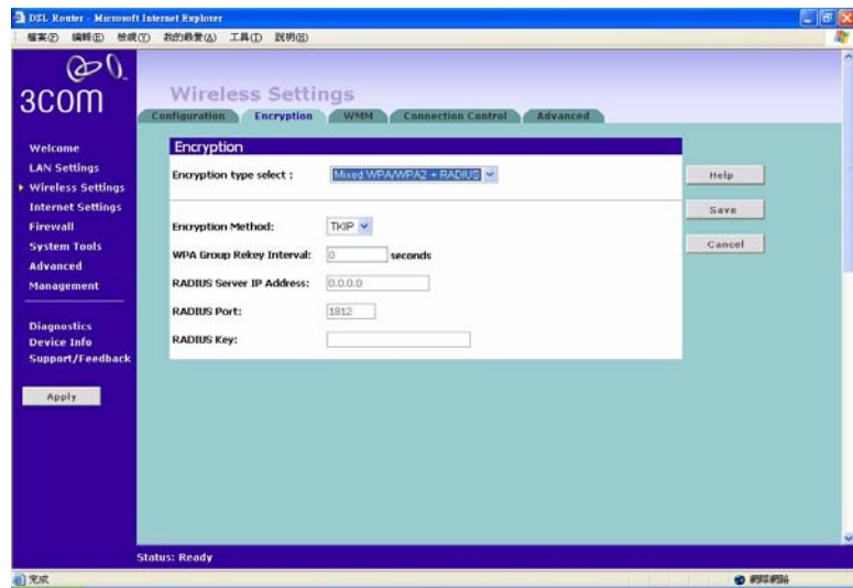
Encryption Figure 32 Encryption Screen
