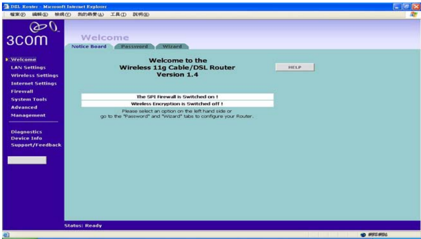
Notice Board Figure 26 Notice Board Screen
