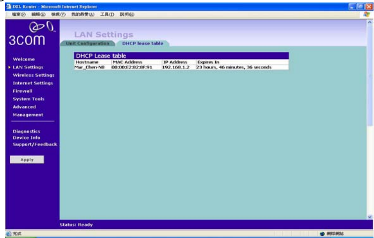
DHCP Lease Table Figure 30 DHCP Lease Table Screen
