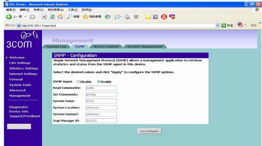
SNMP Figure 57 The SNMP Screen
