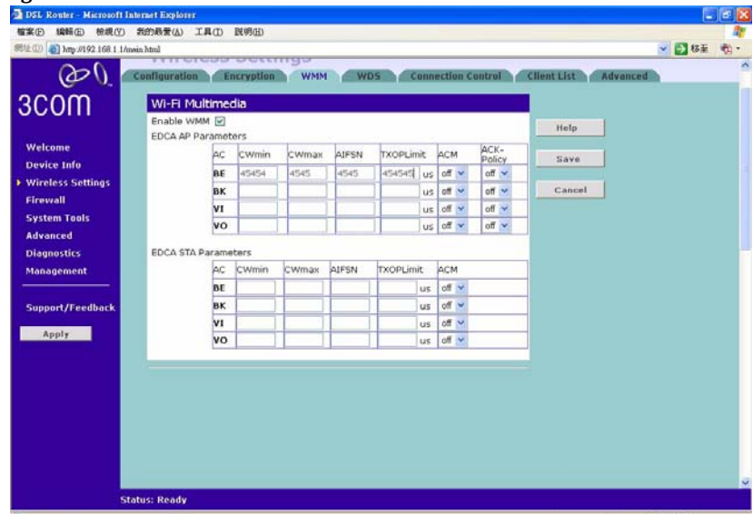
Figure 36 WMM Screen
