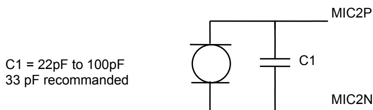
figure 10 : microphone 2 input
