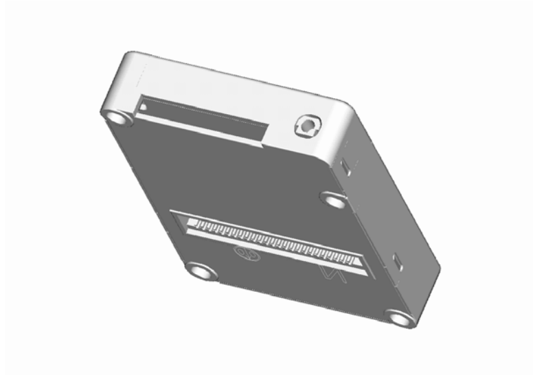
figure 1 : mechanical description
