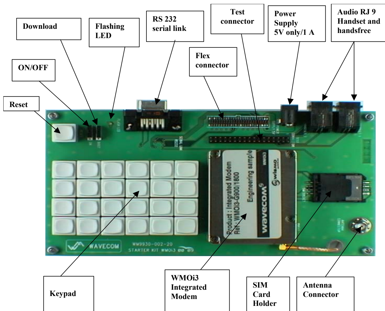
Figure 19: Integra demoboard description
