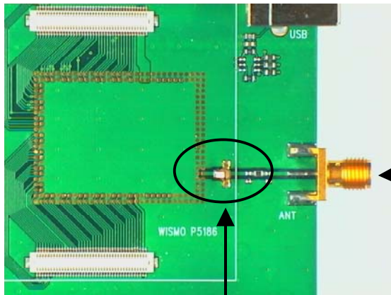
SMA300 Antenna connector
