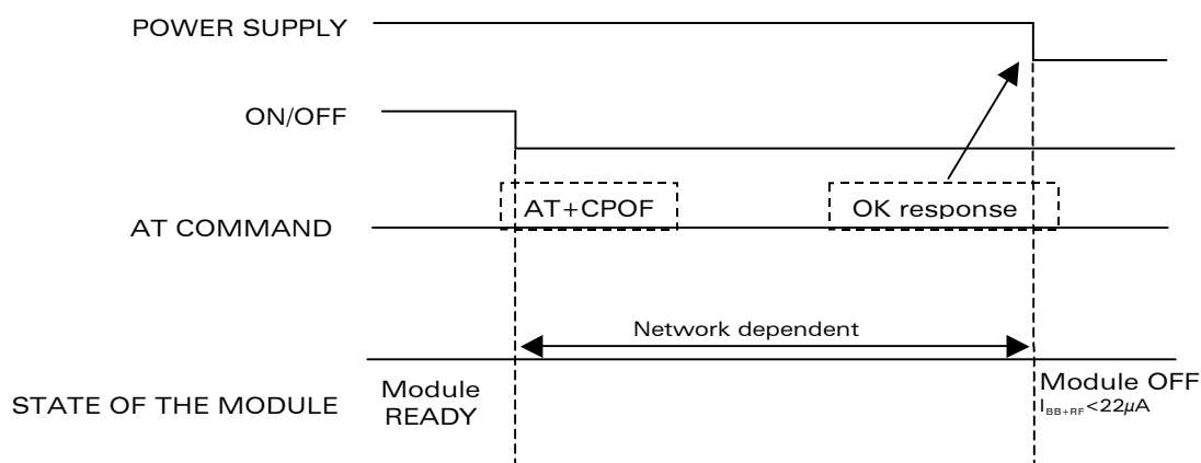
Figure 8 : Power-OFF sequence
