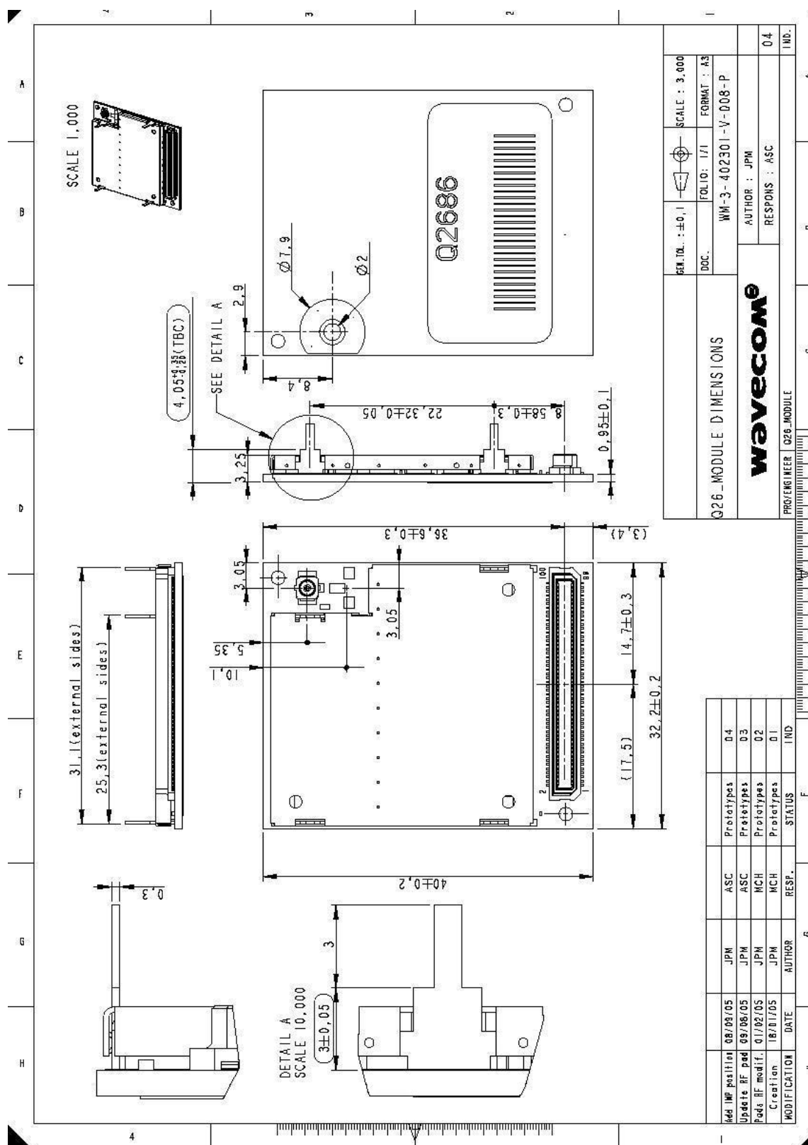
Figure 15 : Mechanical drawing
