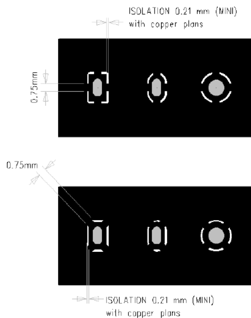
Figure 16 : Layout requirement
