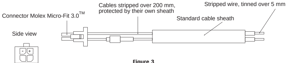
Figure 3 Power supply cable
