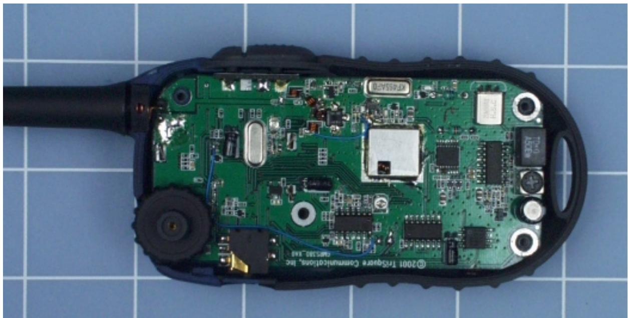
Circuit Board, Top View
