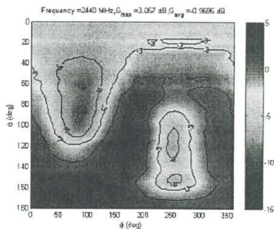
A1.5 – Azimuth gain plot (dBi).
