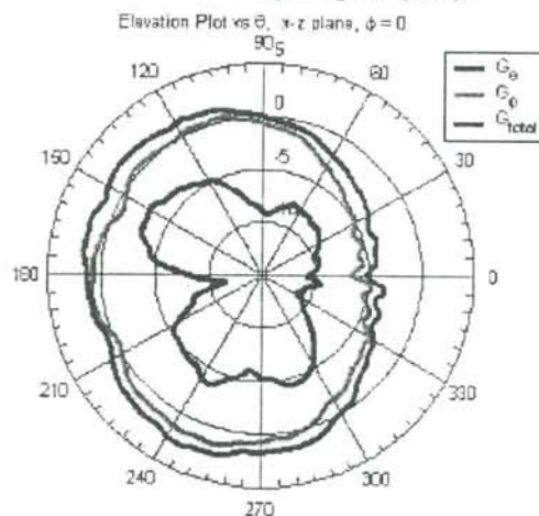
A1.6 – Elevation gain plot (dBi).
