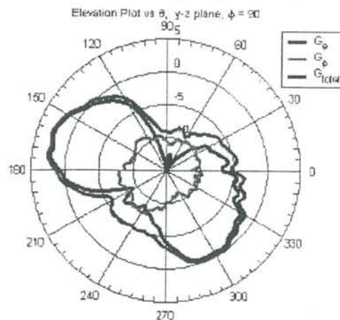
A1.6 – Elevation gain plot (dBi).
