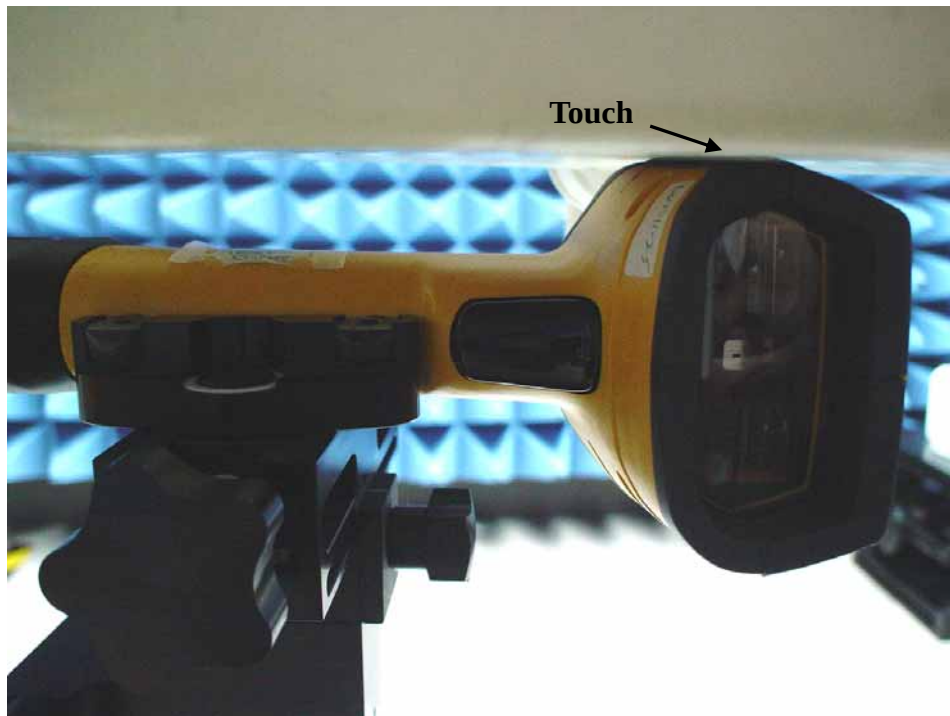
Fig.7 Photo of the EUT Right-side contact to the Flat phantom, Spacing between EUT and phantom –In contact (0mm)
