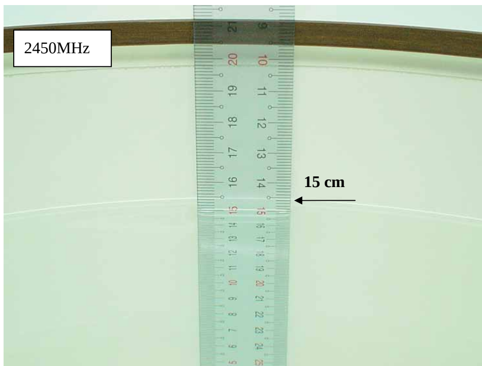
Fig.2 Photograph of the Tissue Simulate Fluid liquid depth 15cm for Flat phantom
