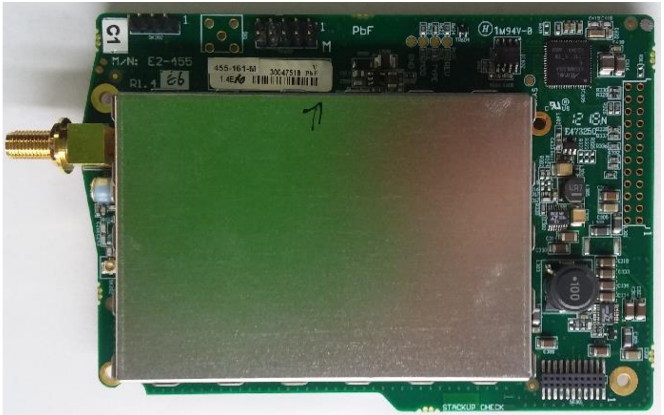
Top Side – Outer Shield Removed
