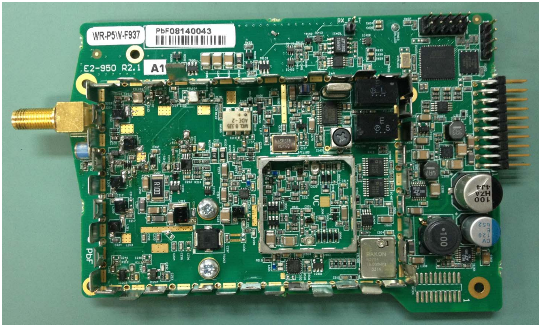
Additional internal photo with the VCO shield removed
