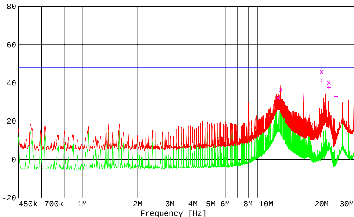
Quasi-Peak Measurements
