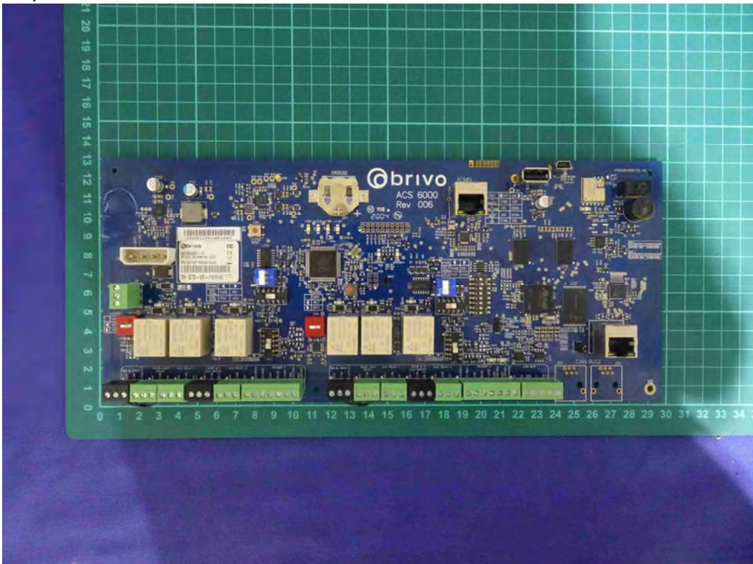
(234) EUT Photo – M/N: ACS6000, B-ACS6000, B-ACS6000-A, B-ACS6000-E, B-ACS6000-S
