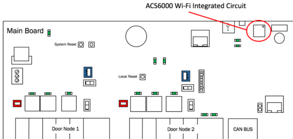
Figure 25 - ACS6000 Wi-Fi Integrated Circuit Location
