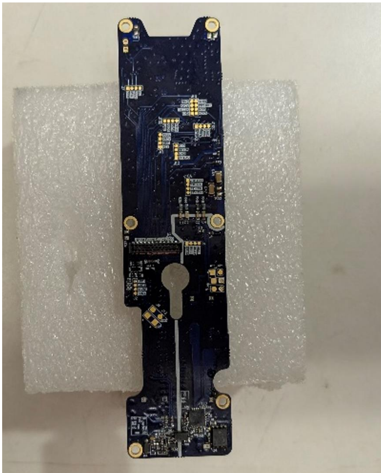
Photograph 8 – Bottom view of Power PCBA
