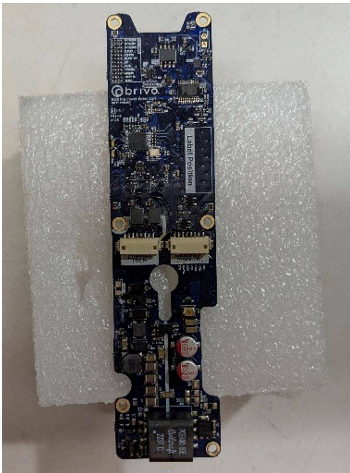
Photograph 7 – Top view of Power PCBA
