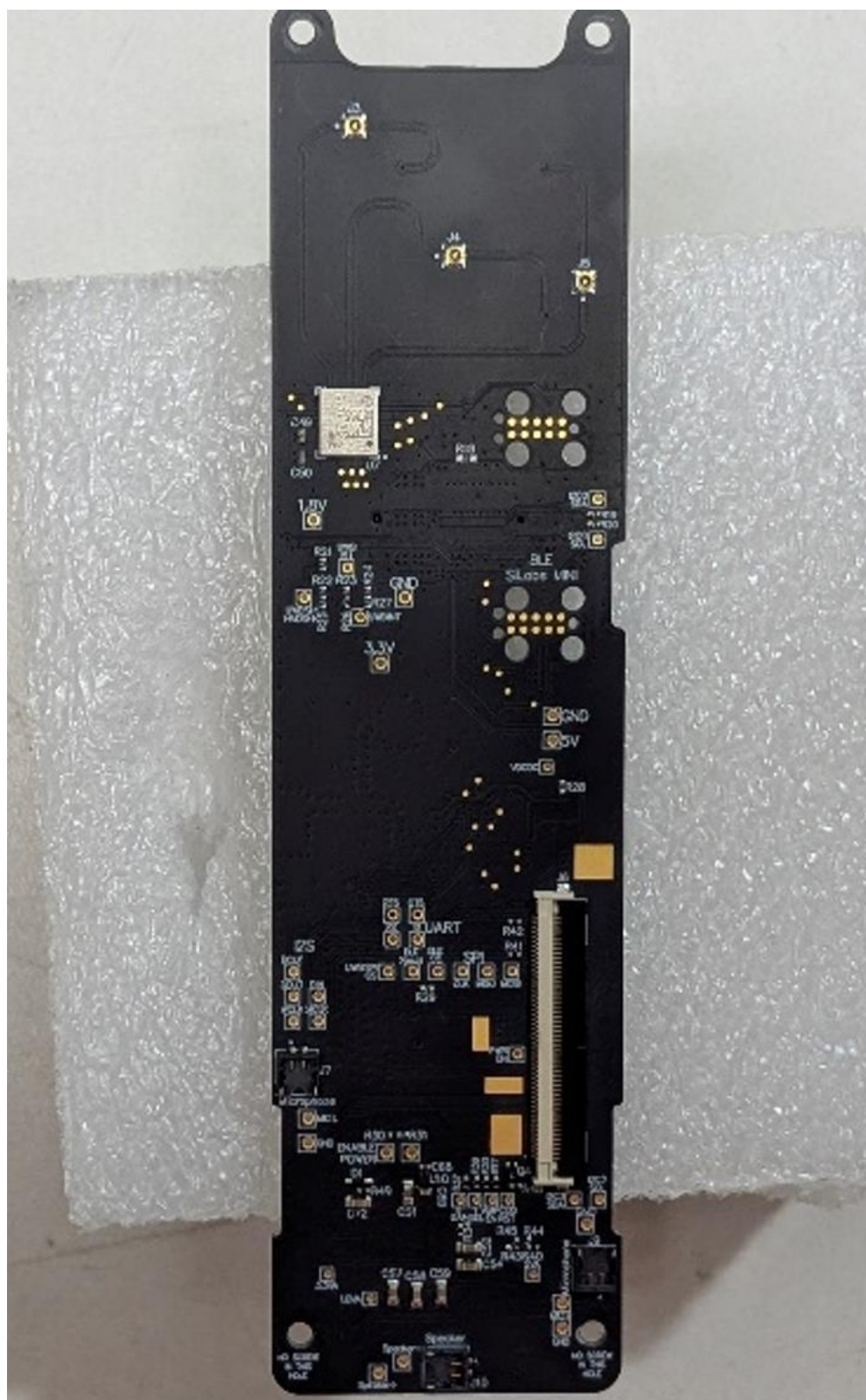
Photograph 4 – Bottom view of RF PCB
