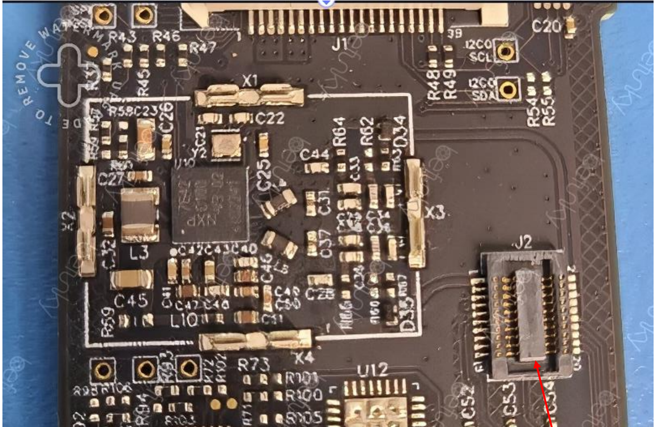
Photograph 1 –View of the RF Circuitry under the RF Shield, NFC
