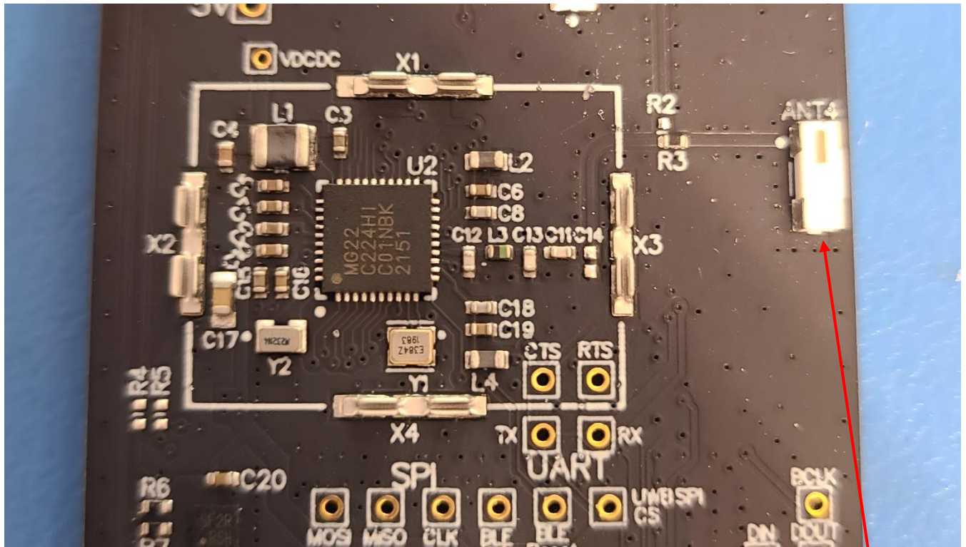
Photograph 2 –View of the RF Circuitry under the RF Shield, BLE
