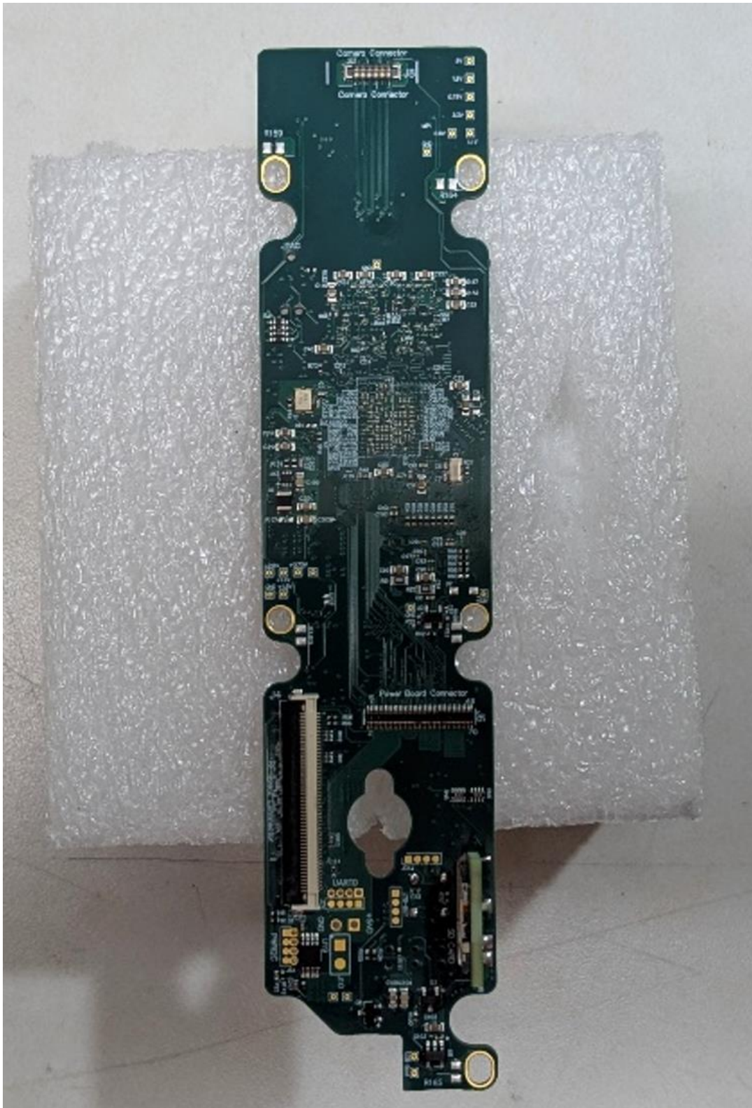
Photograph 9 – Top view of Main PCBA
