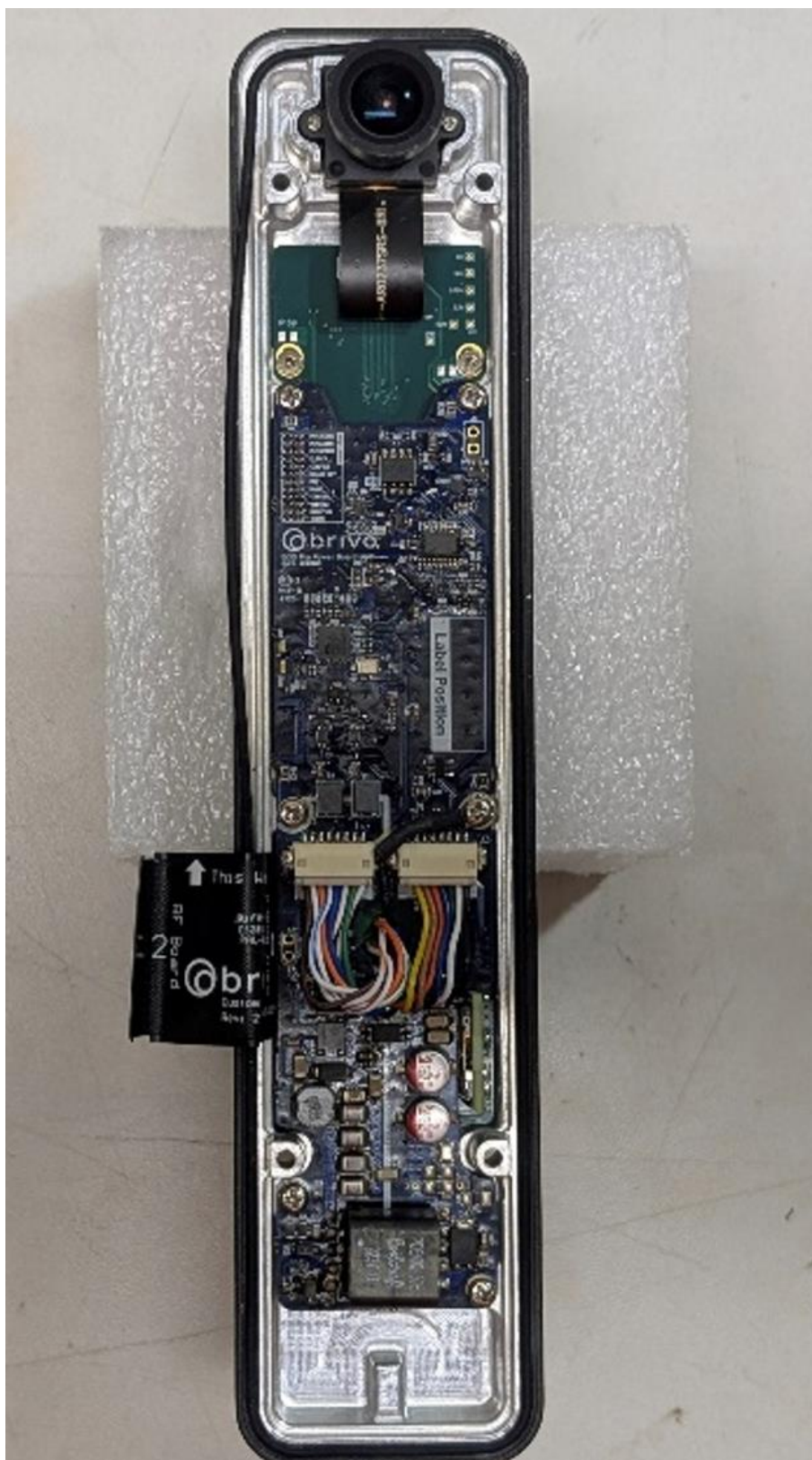
Photograph 16 – Back housing with Power PCB on top of Main PCB
