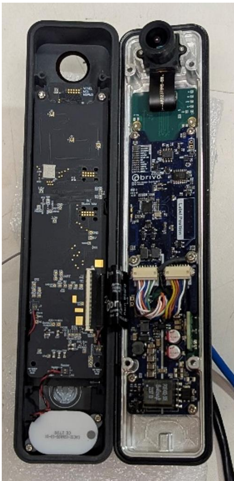
Photograph 17 – Front and Back housings with all PCBs installed
