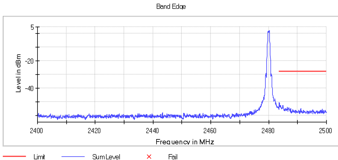
Graph 8: Upper Band Edge Plot
