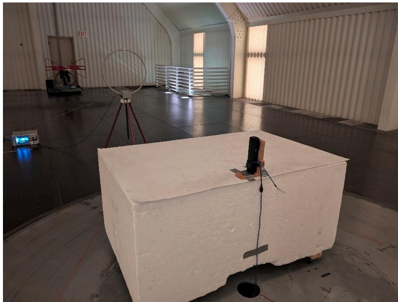
Photograph 4: Back View Radiated Emissions Worst Case Configuration – Frequencies Below 30 MHz
