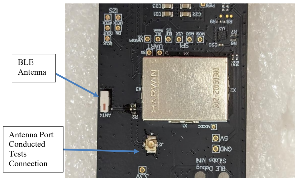
Photograph 24: Closeup View of BLE Circuitry on Front of "RF Board"
