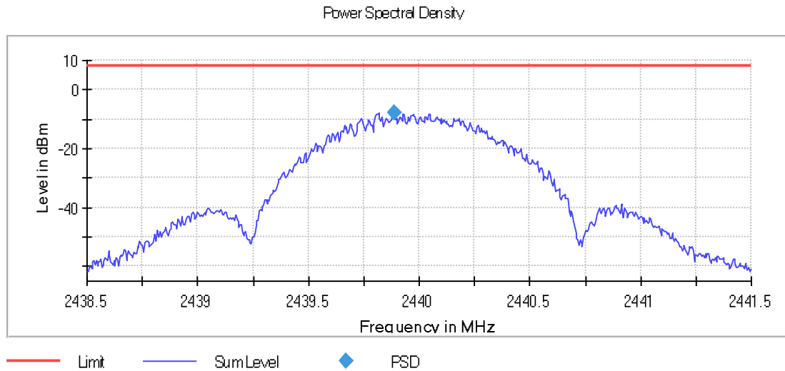
Graph 12: Middle Channel 100 kHz PSD Plot
