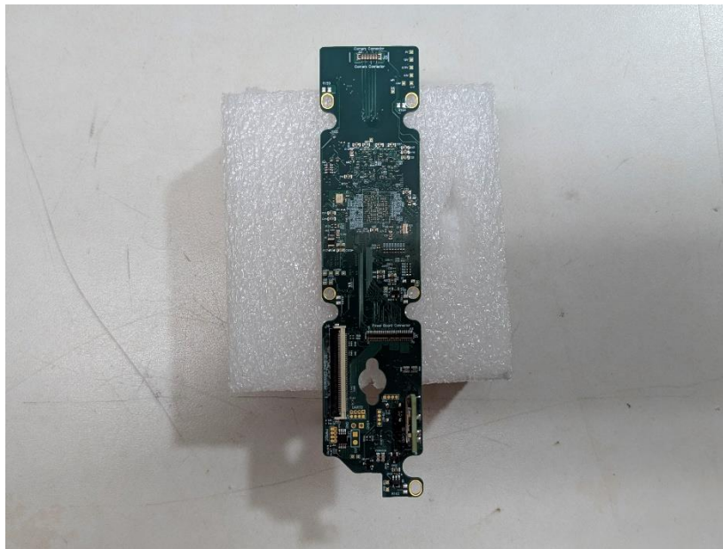
Photograph 38: Front of PCB "Main Board"
