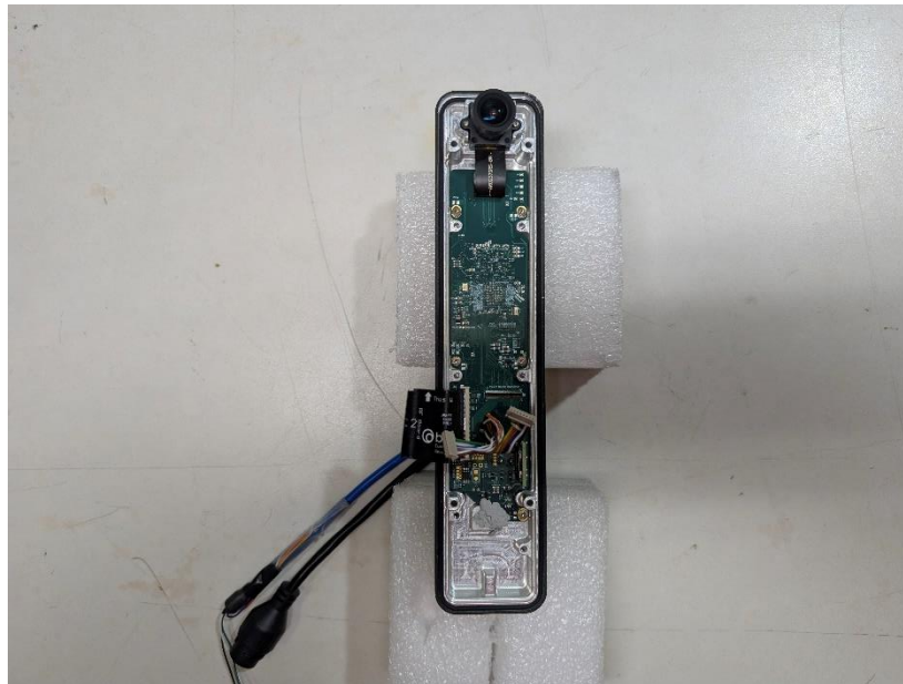
Photograph 17: Enclosure Back Showing Placement of “Main Board” with “Power Board” Removed
