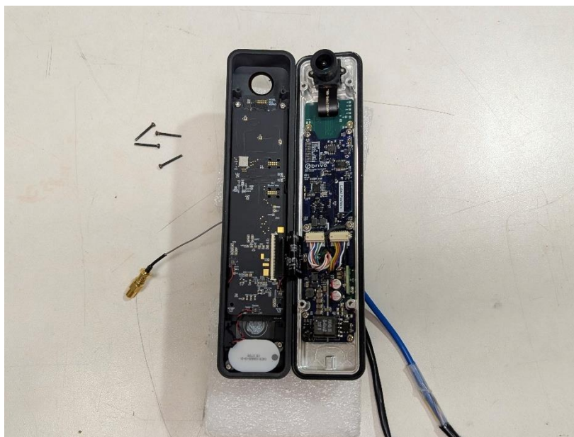
Photograph 9: Rear Cover Removed Showing Placement of PCBs in Enclosure (“RF Board” on Top of “Keypad Board” on Left, “Power Board” on Top of “Main Board” on Right)
