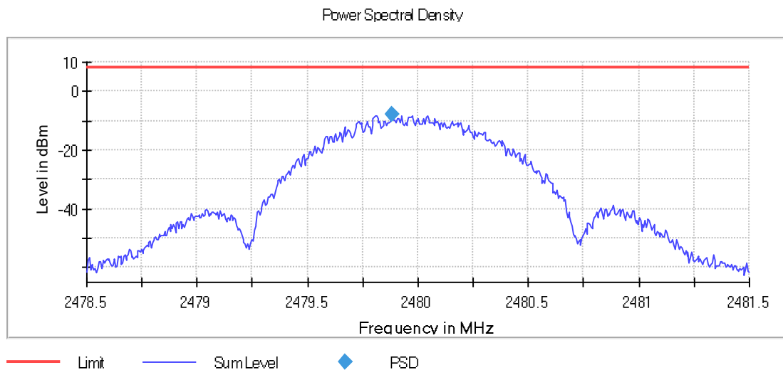
Graph 13: Highest Channel Output 100 kHz PSD Plot
