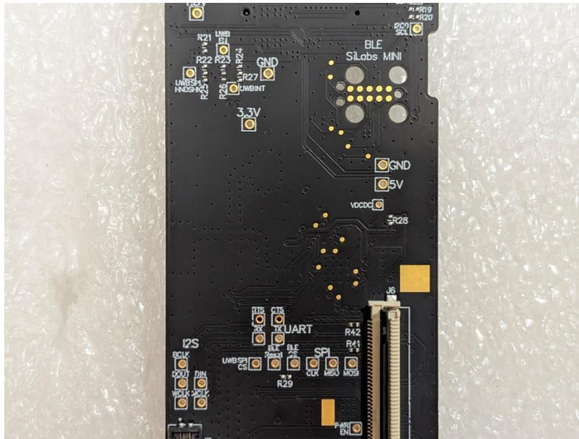
Photograph 25: Closeup View of BLE Circuitry on Front of “RF Board”
