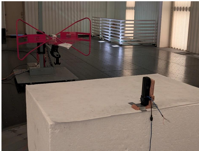
Photograph 6: Back View Radiated Emissions Worst Case Configuration – Frequencies 30 - 1000 MHz
