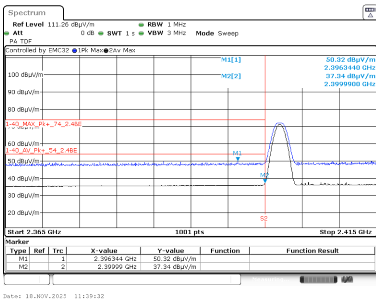
Graph 9: Radiated Lower Band Edge Plot
