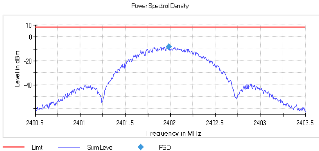
Graph 11: Lowest Channel 100 kHz PSD Plot
