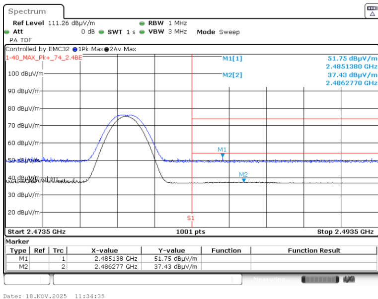
Graph 10: Radiated Upper Band Edge Plot
