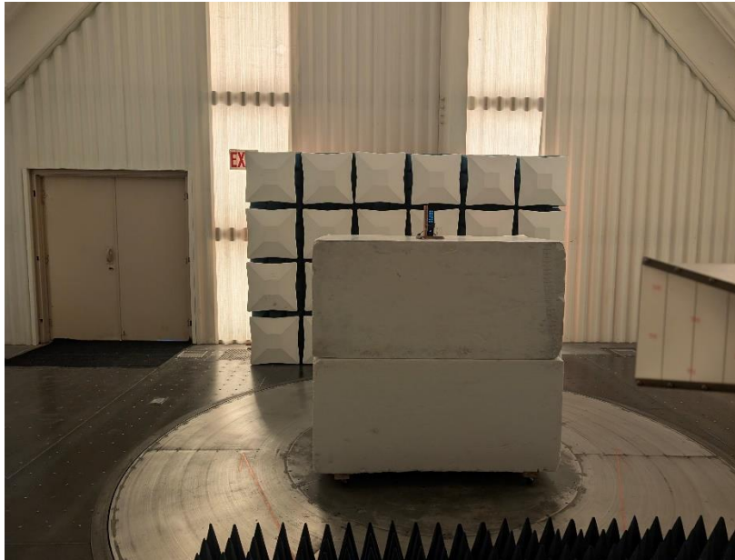
Photograph 1: Front View Radiated Emissions Worst Case Configuration – Frequencies Above 1000 MHz
