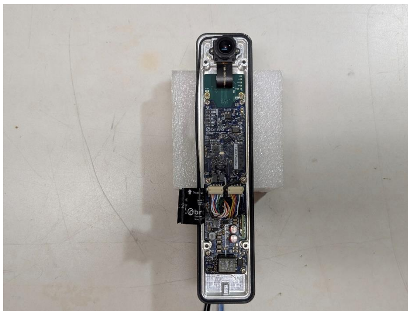
Photograph 16: Enclosure Back Showing "Power Board" on Top of "Main Board"
