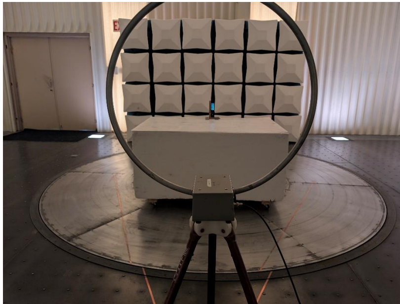
Photograph 3: Front View Radiated Emissions Worst Case Configuration – Frequencies Below 30 MHz
