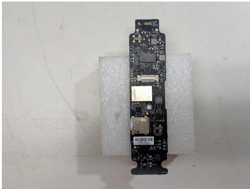
Photograph 26: Front of PCB “Keypad Board”
