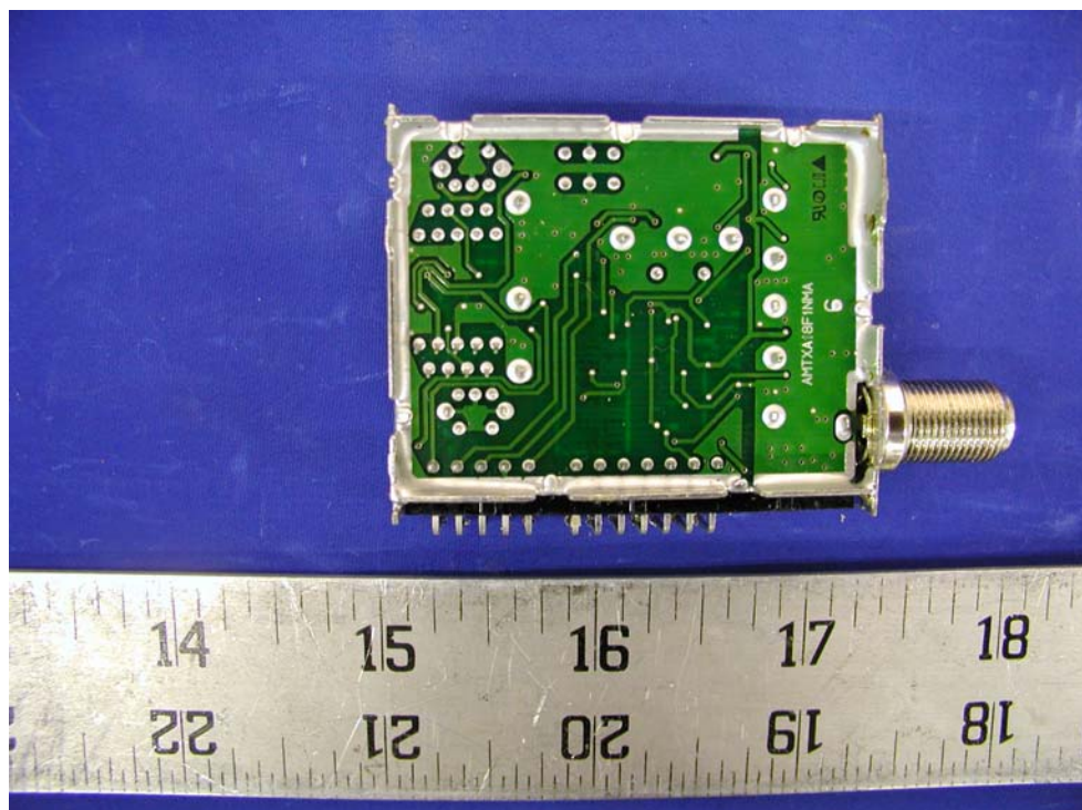
RF Board - Solder View
