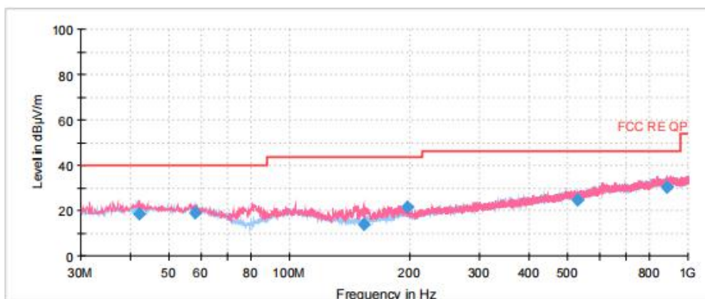
Radiated Emission from 30MHz to 1GHz
