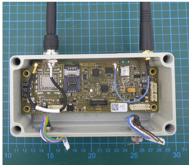
Host Internal view
