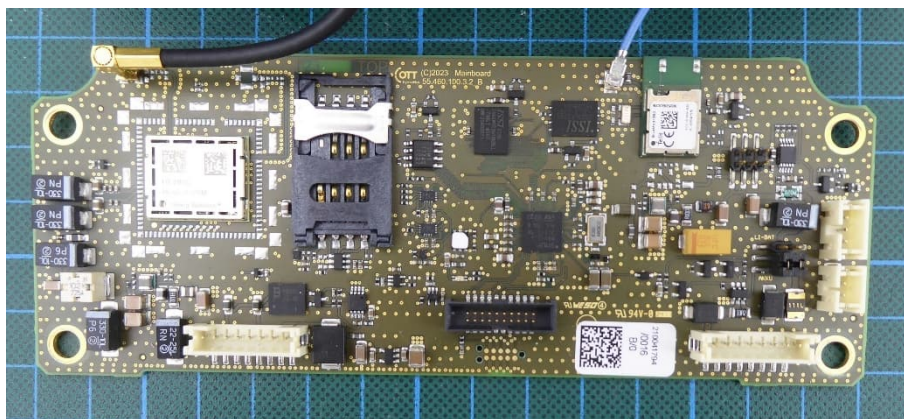
Host PCB Top view
