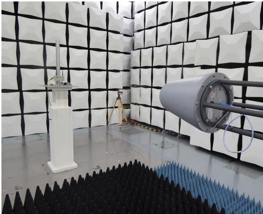
Test setup SAC from 1 GHz to 4 GHz
