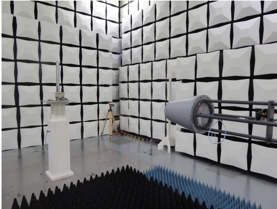
Test setup SAC from 4 GHz to 18 GHz
