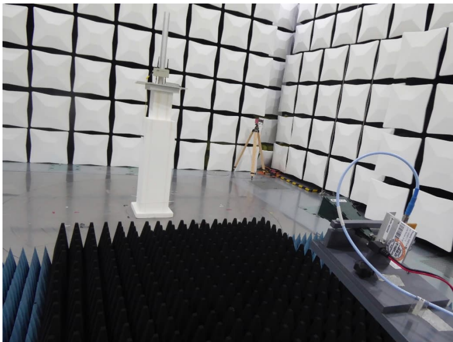
Test setup SAC from 18 GHz to 26.5 GHz
