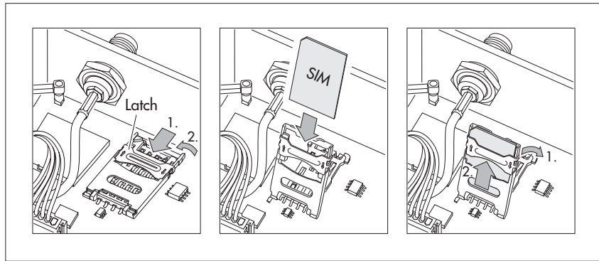
Fig. 3: Insert SIM card into the SIM card holder of the OTT SensorLink 1000.
