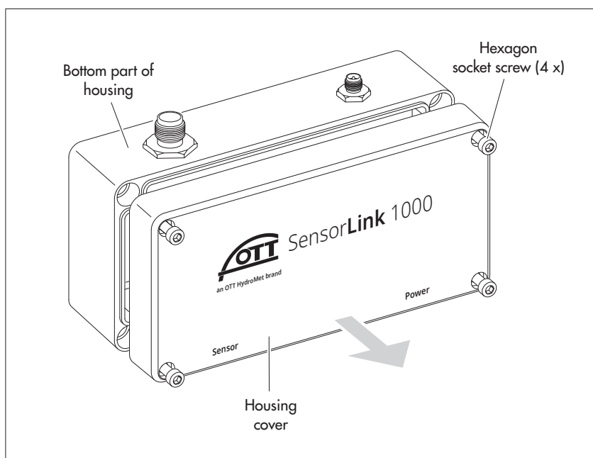
Fig. 2: Remove the housing cover of the OTT SensorLink 1000.
