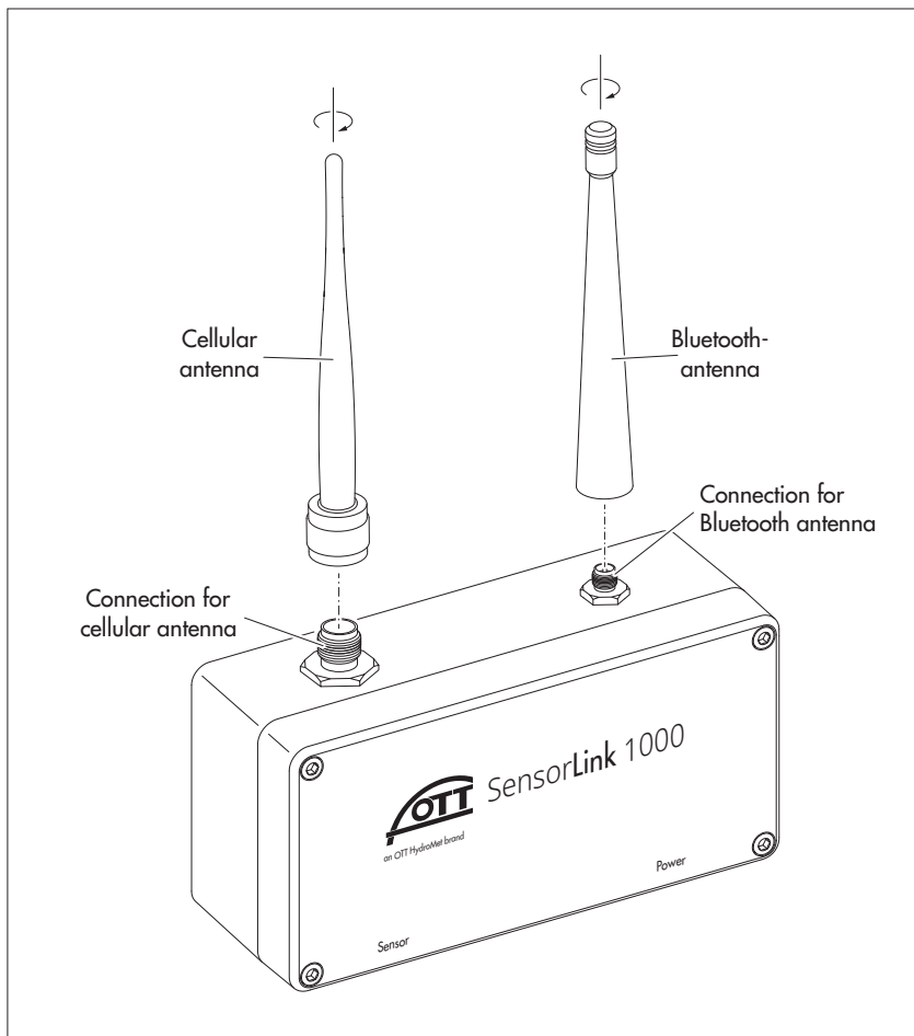
Fig. 4: connecting the cellular- and Bluetooth antenna with the OTT SensorLink 1000.
