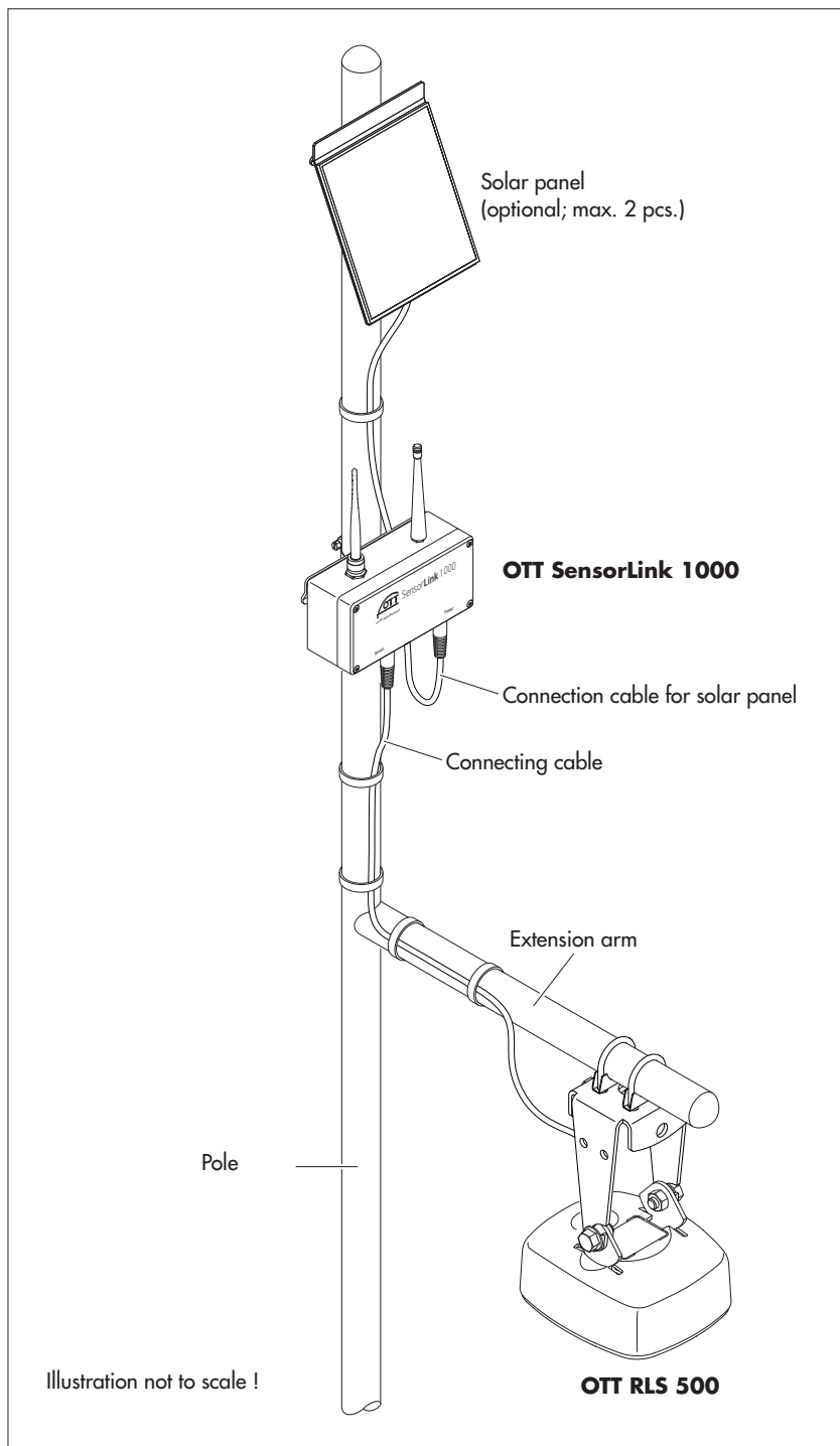
Fig. 8: Example installation of an autonomous level measuring station; consisting of a compact datalogger OTT SensorLink 1000, radarsensor OTT RLS 500 and an optional 5 watt solar panel.
