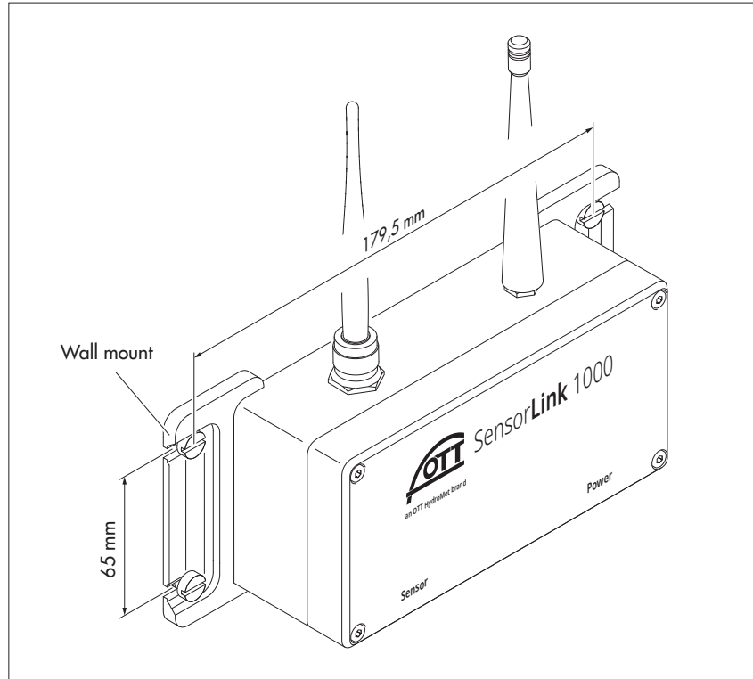
Fig. 5: mounting the OTT SensorLink 1000 housing – Variant A.
