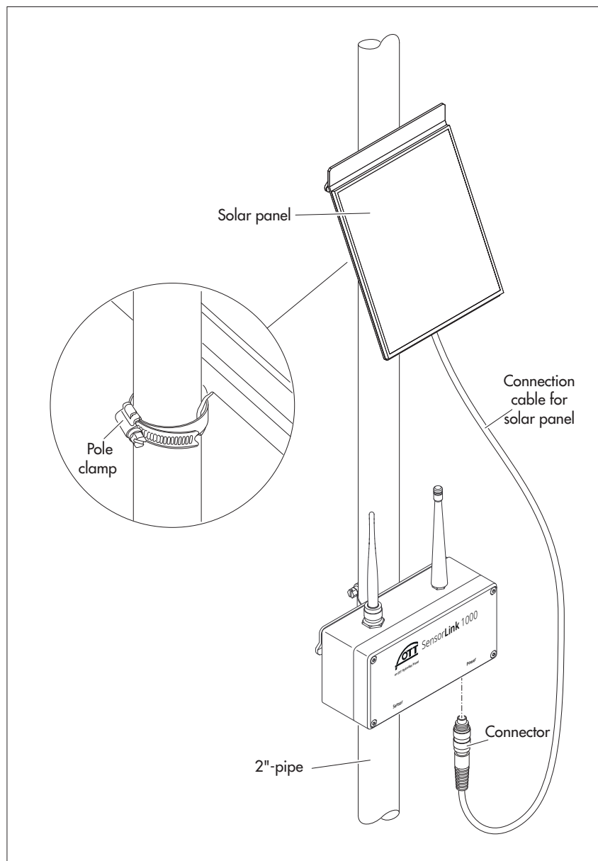
Fig. 9: mounting the solar panel and connecting it to the OTT SensorLink 1000.
