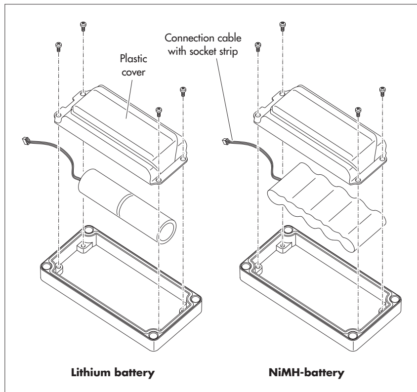
Fig. 12: exchange the lithium battery/NiMH rechargeable battery.
