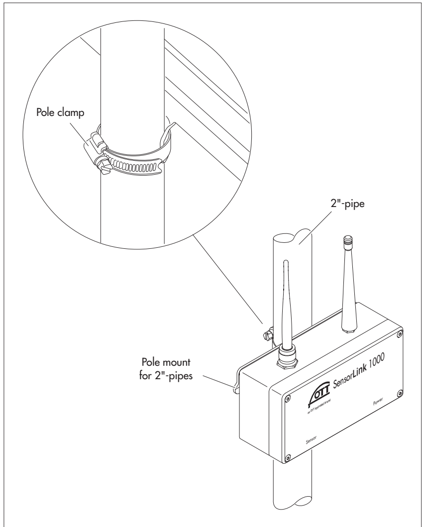
Fig. 6: mounting the OTT SensorLink 1000 housing – Variant B.
