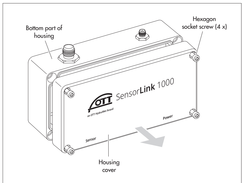
Fig. 10: removing the housing cover of the OTT SensorLink 1000.
