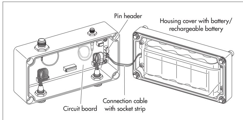
Fig. 11: open housing of the OTT SensorLink 1000.
