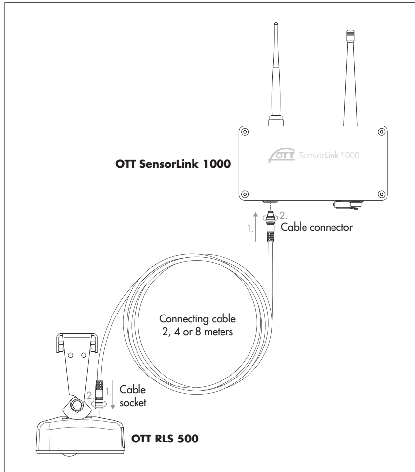
Fig. 7: Connecting the OTT RLS 500 to the OTT SensorLink 1000.
