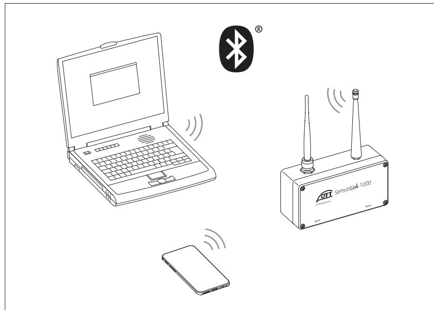
Fig. 13: communication connection between PC/mobile device and OTT SensorLink 1000 via Bluetooth.
