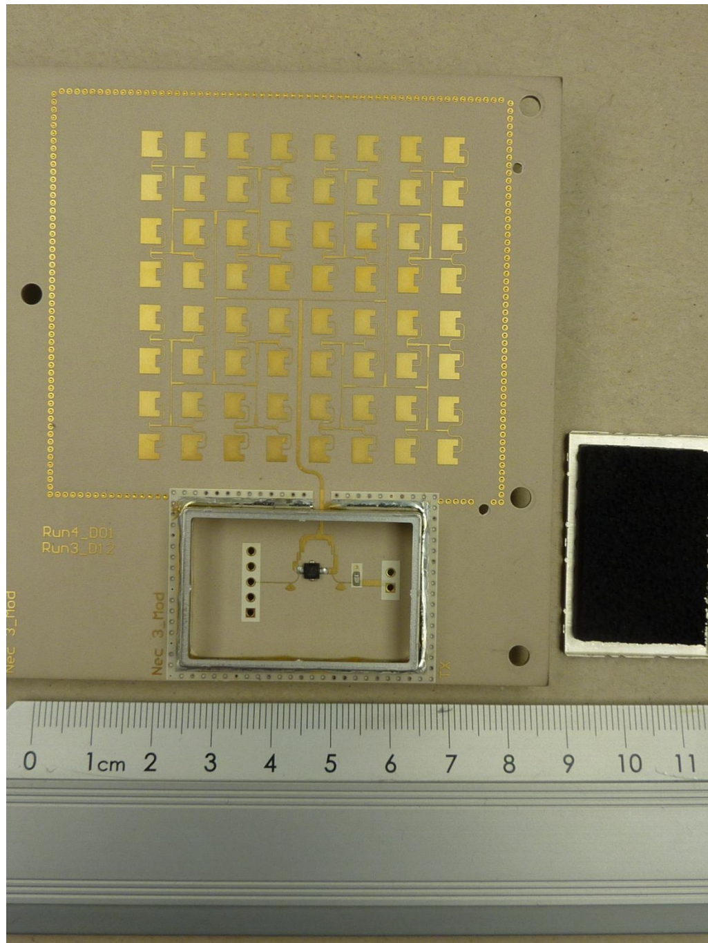
143563_k.JPG: RLS, detail view to TX patch and shielding cover
