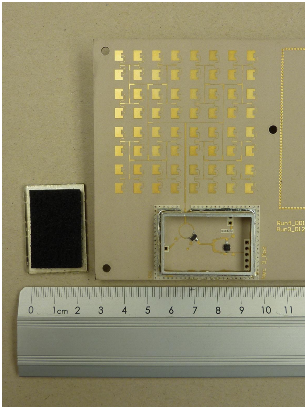
143563_I.JPG: RLS, detail view to RX patch and shielding cover
