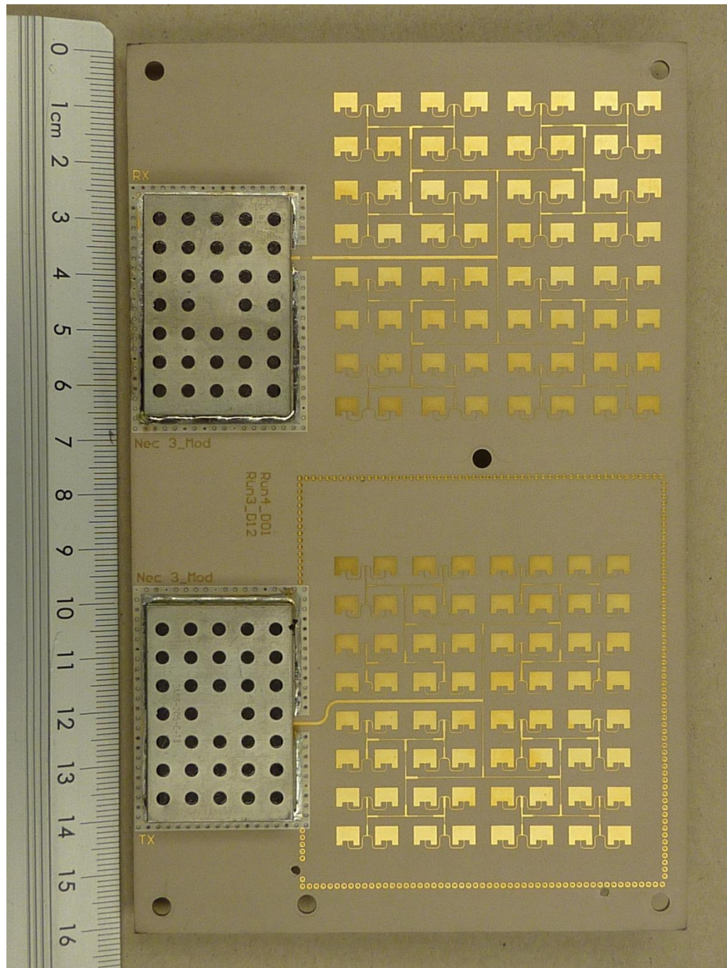
143563_j.JPG: RLS, PCB, bottom view
