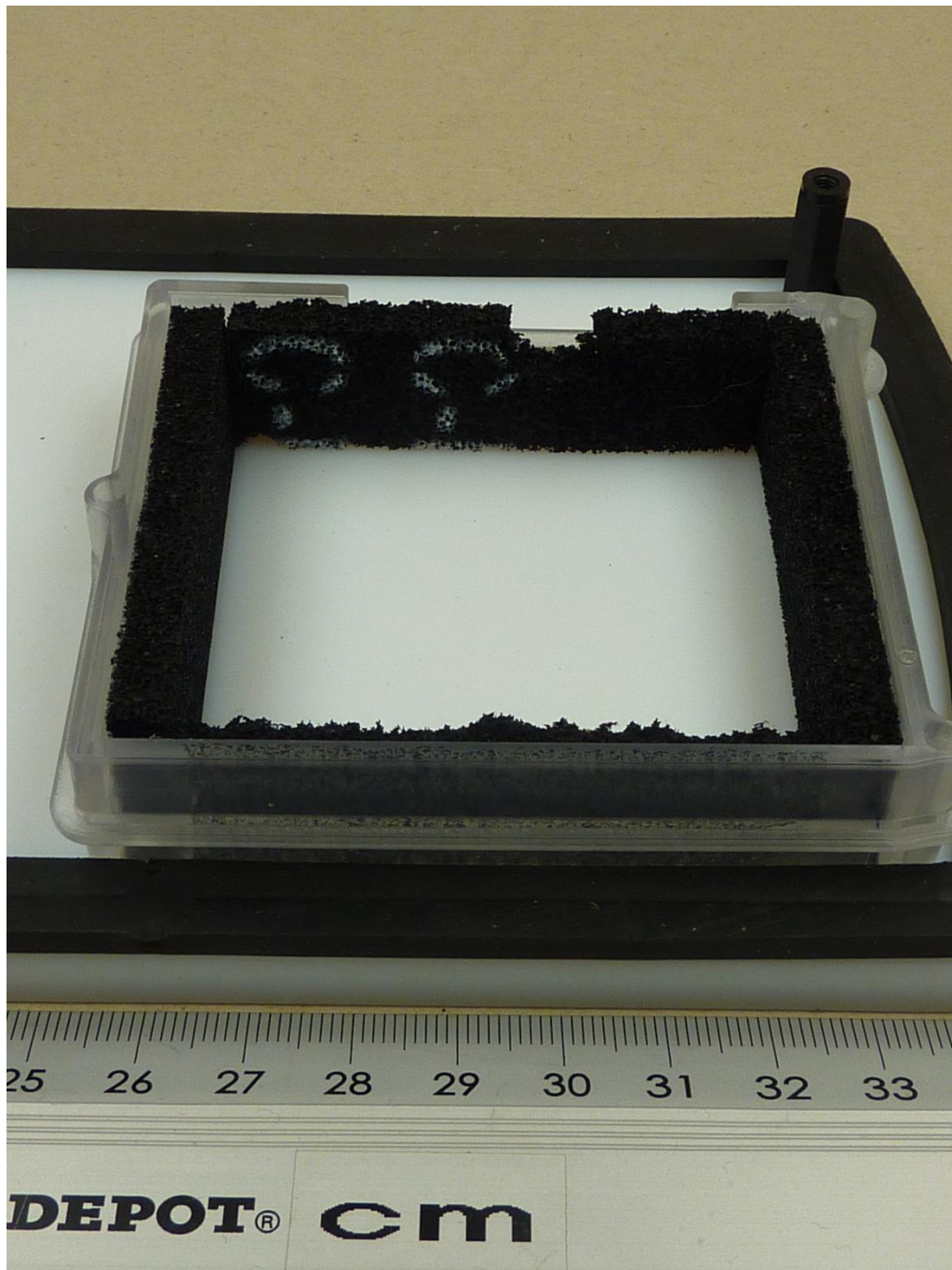
143563_h.JPG: RLS, internal view 2 (absorbing material for TX patch)
