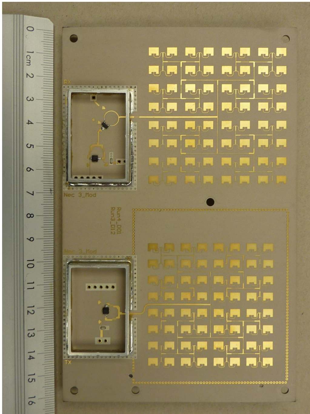
143563_m.JPG: RLS, PCB, bottom view (shielding cover removed)
