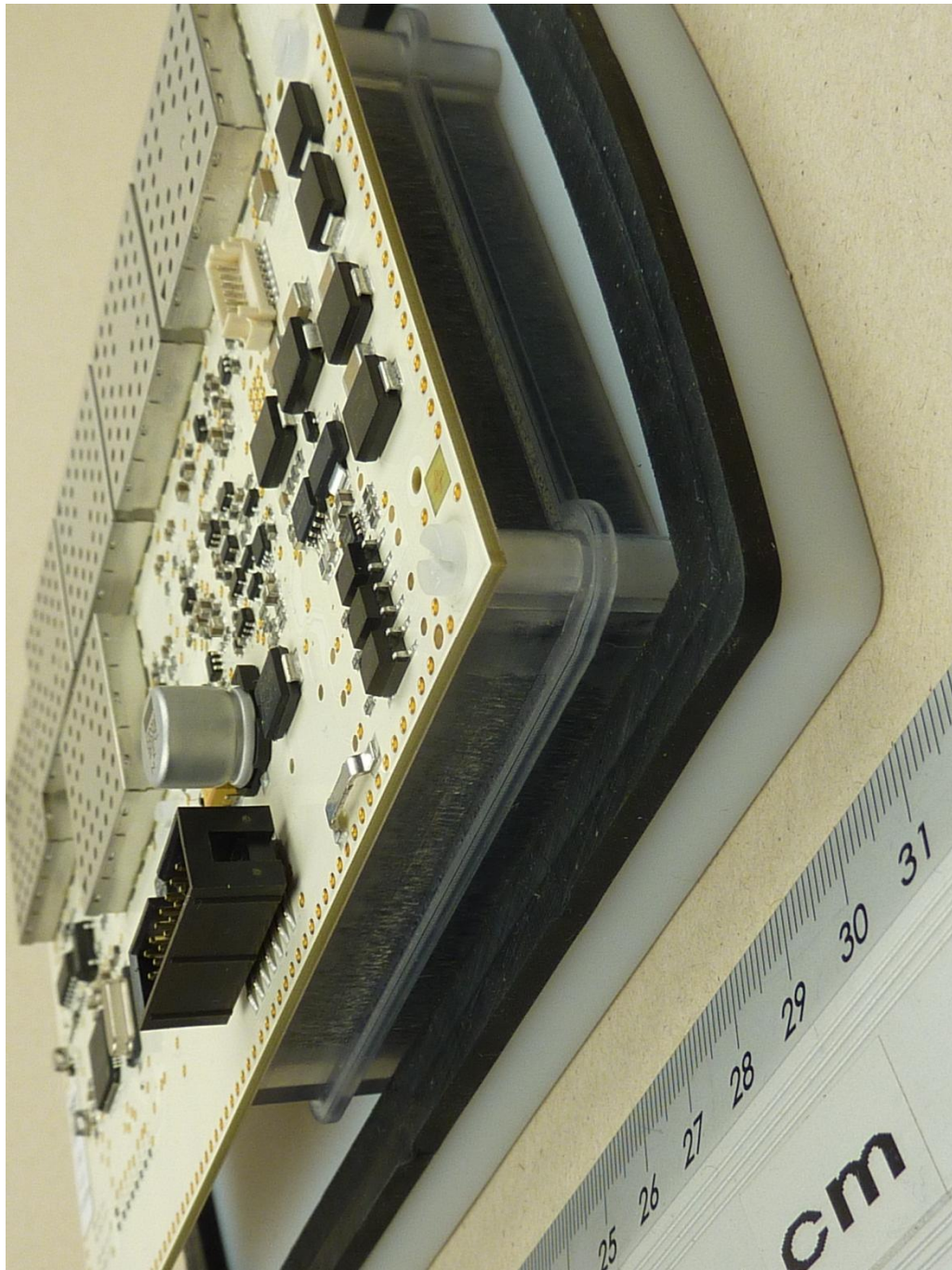
143563_f.JPG: RLS, internal view 1 (cover removed)
