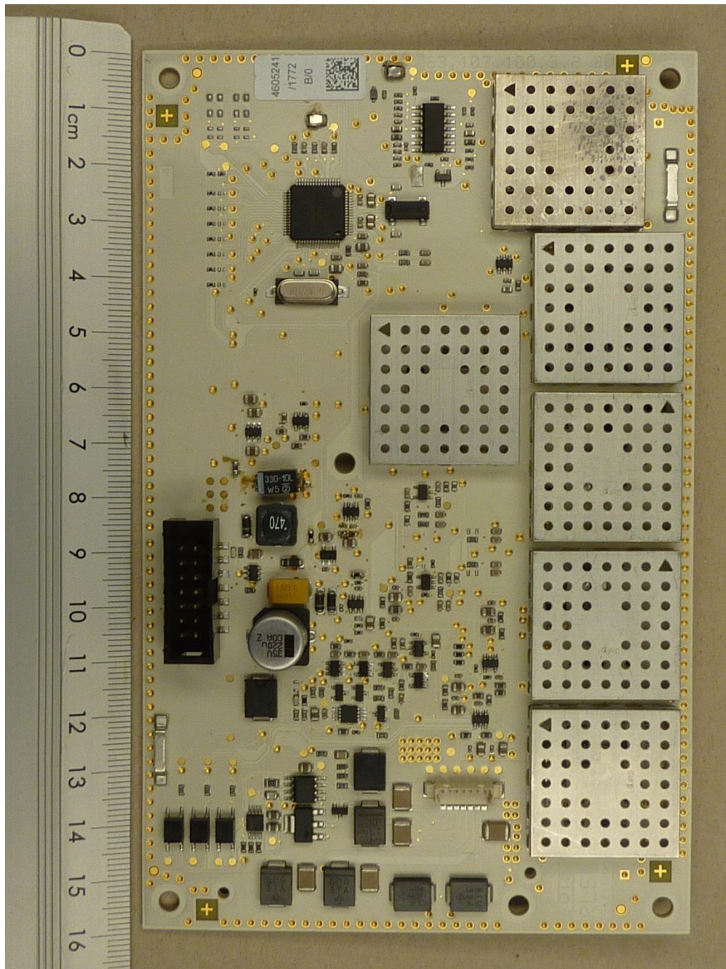
143563_i.JPG: RLS, PCB, top view
