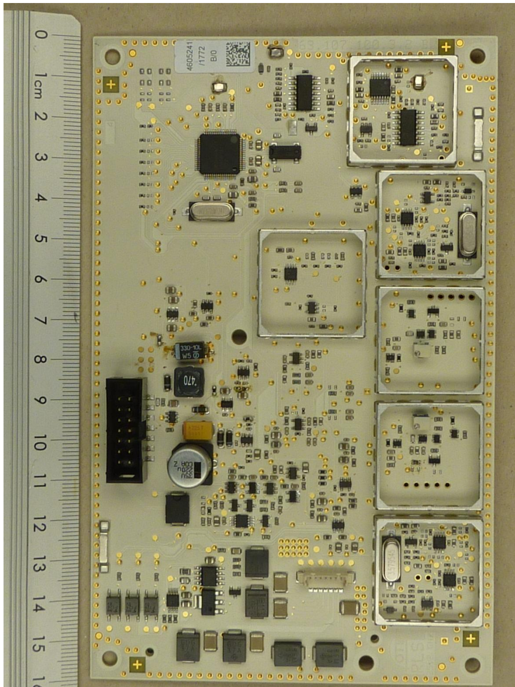
143563_n.JPG: RLS, PCB, top view (shielding cover removed)
