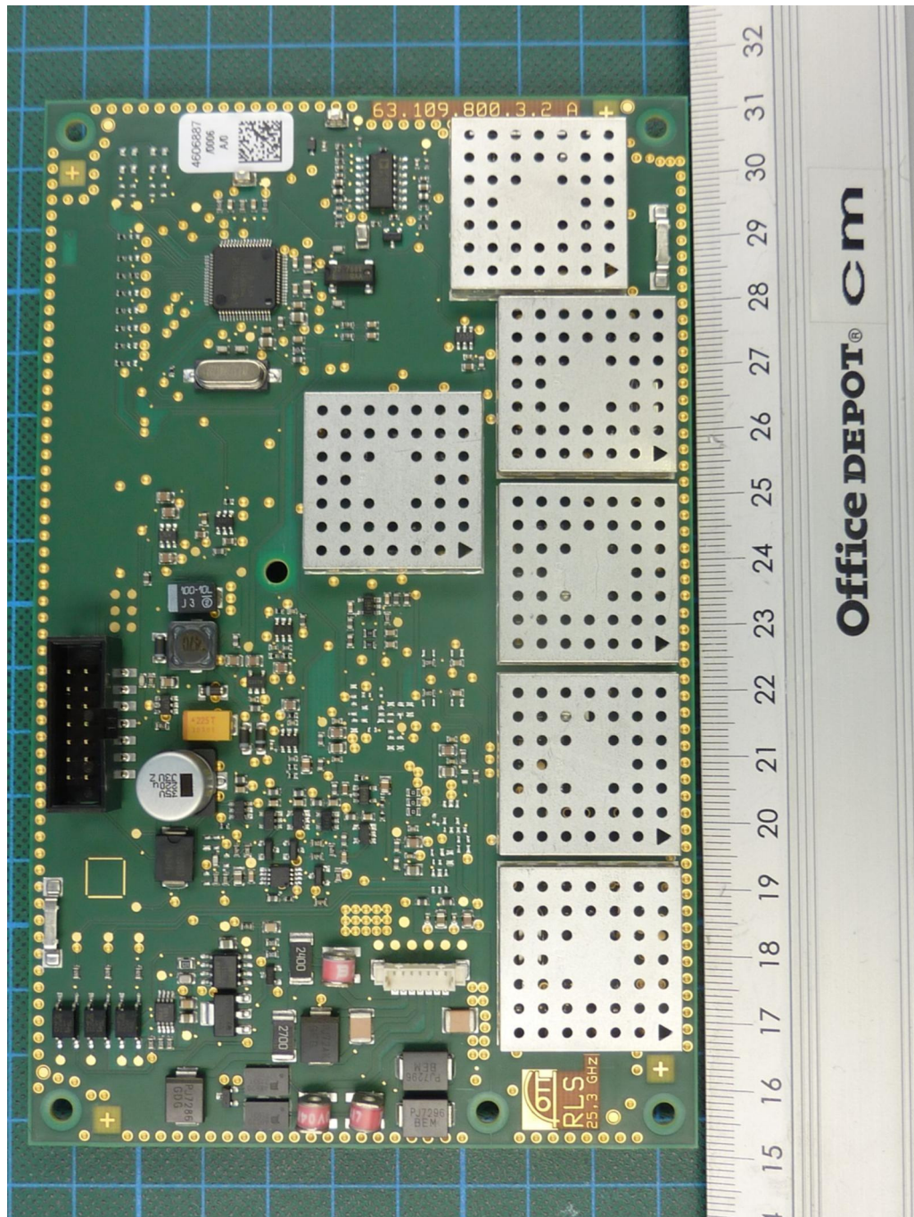
172171_h.JPG: RLS, PCB, top view
