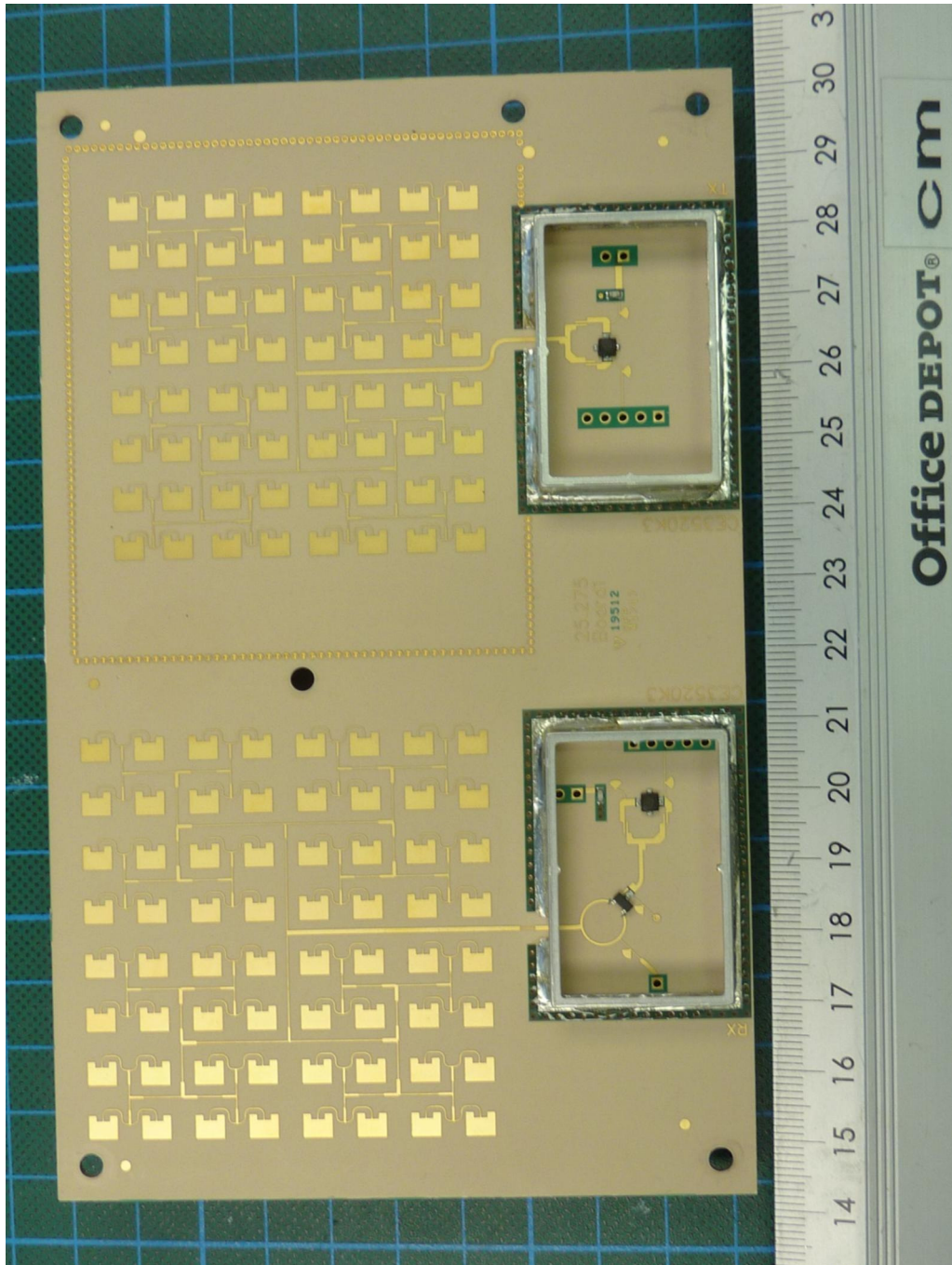
172171_k.JPG: RLS, PCB, bottom view, shielding removed
