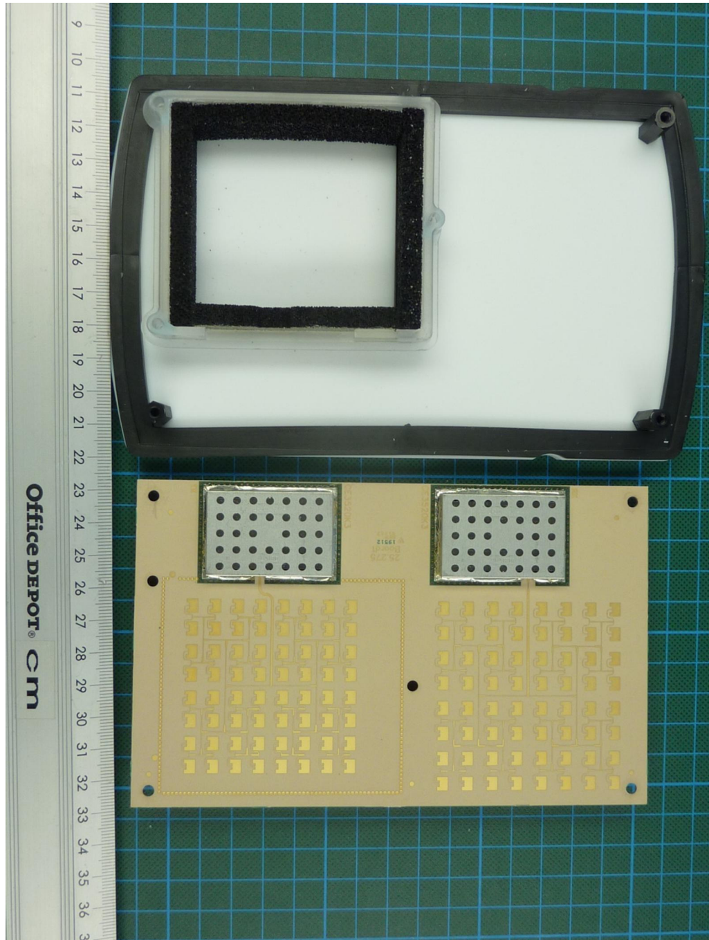
172171_f.JPG: RLS, internal view 2
