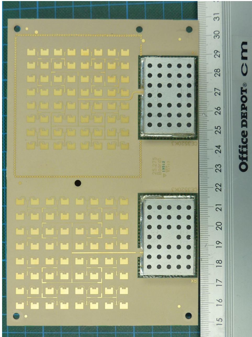
172171_j.JPG: RLS, PCB, bottom view
