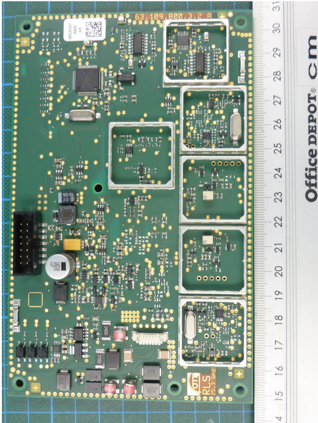
172171_i.JPG: RLS, PCB, top view, shielding removed
