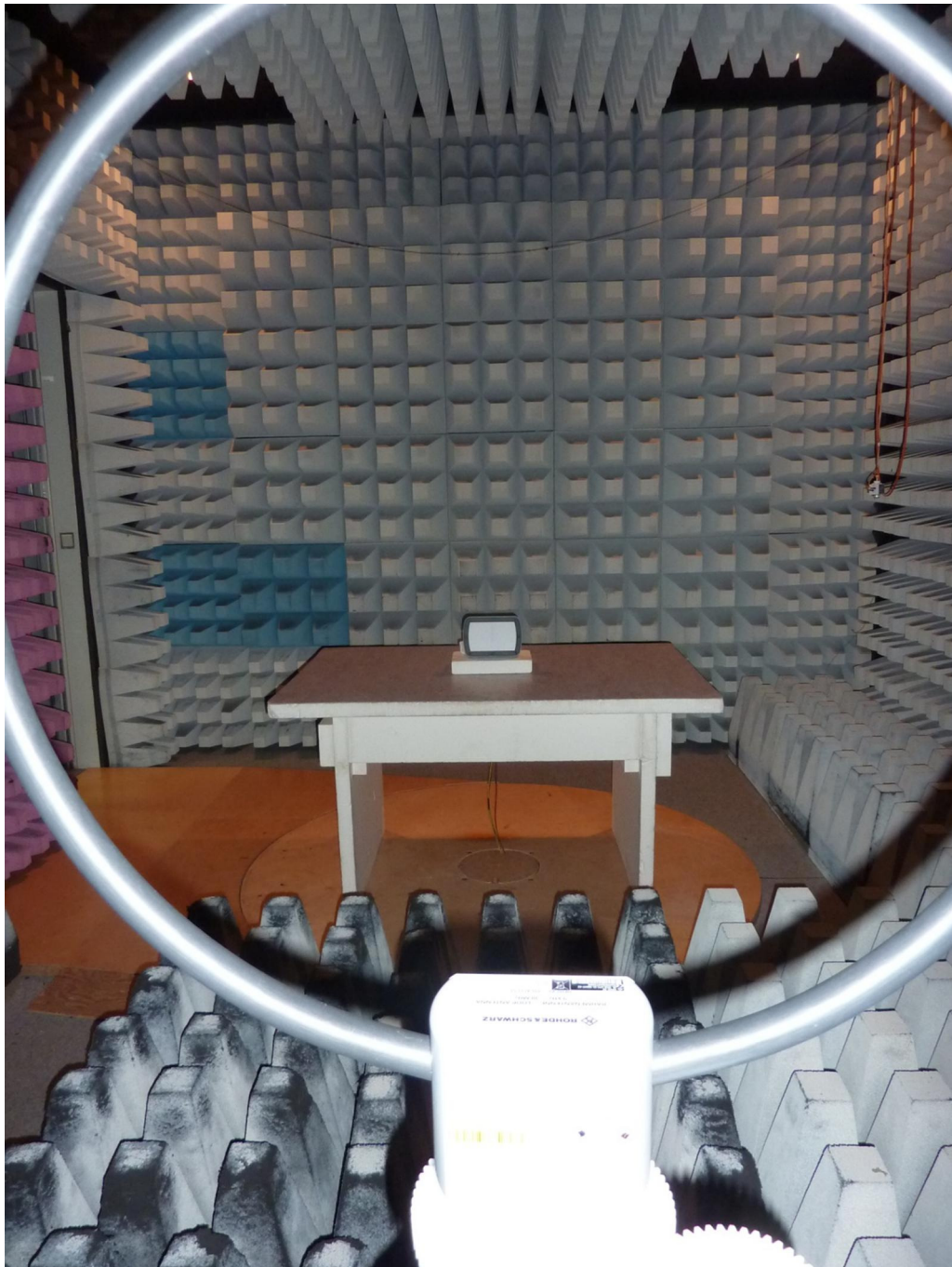
172171_3.JPG: RLS, test setup fully anechoic chamber
