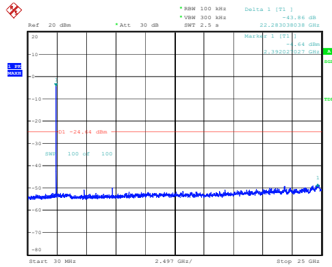
BLE_1M_Low_Channel
