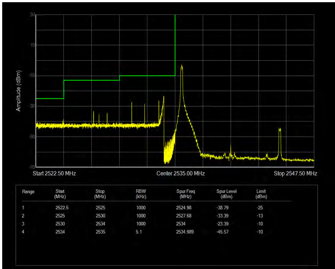
Band41 16QAM BW=5MHz Channel=40065 RB Size=1 Position=#Max
