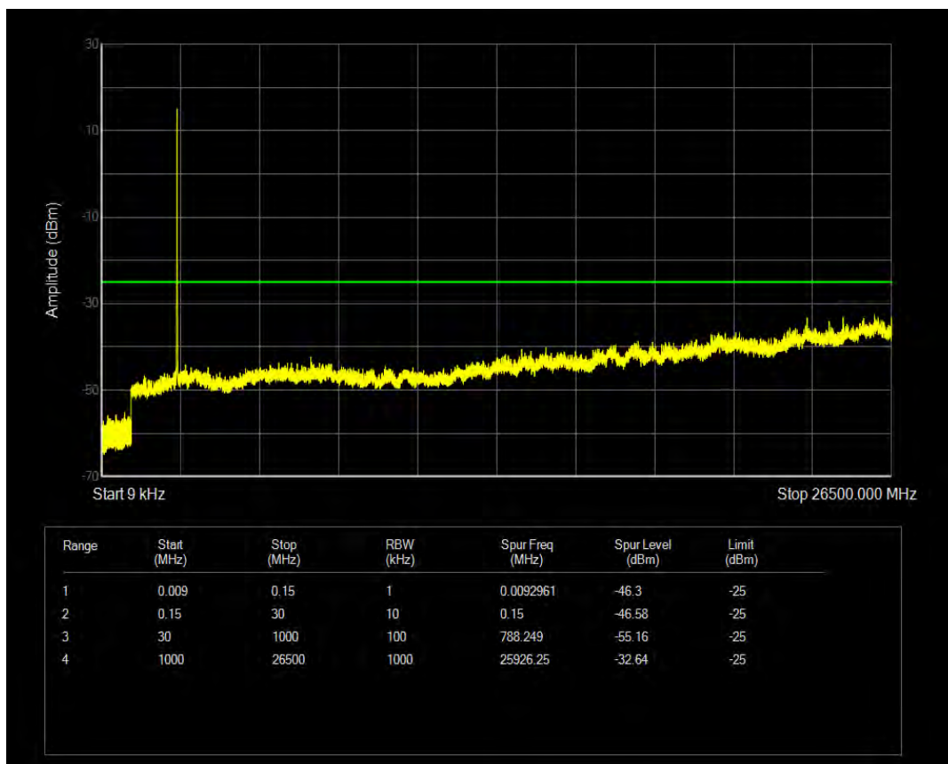
Band41 16QAM BW=10MHz Channel=40740 RB Size=1 Position=#0
