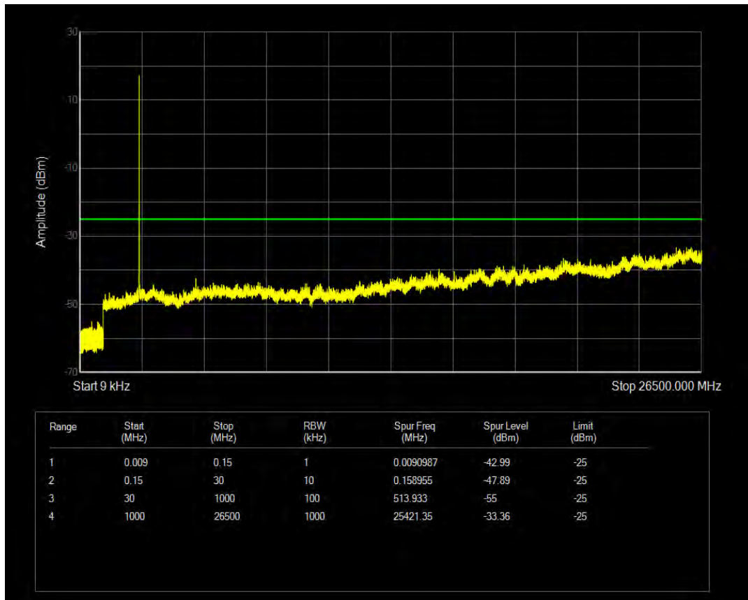
Band41 16QAM BW=20MHz Channel=41340 RB Size=1 Position=#0
