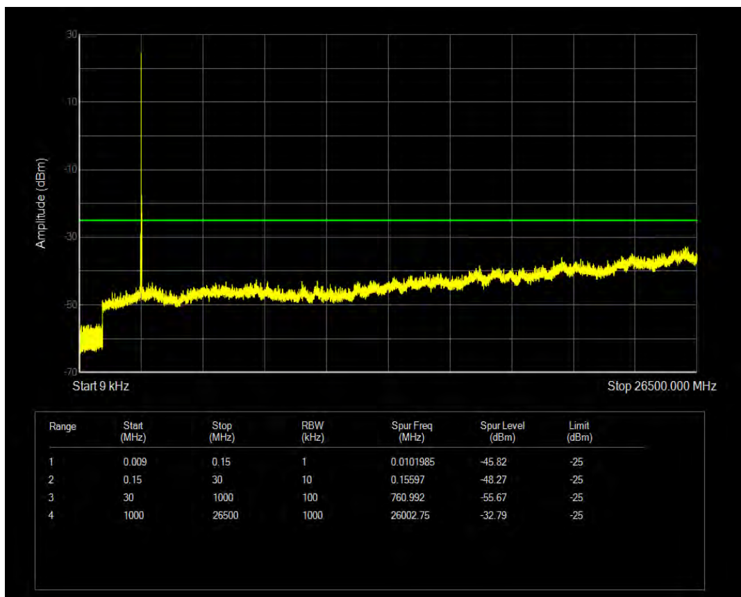
Band41 16QAM BW=15MHz Channel=40115 RB Size=75 Position=#0
