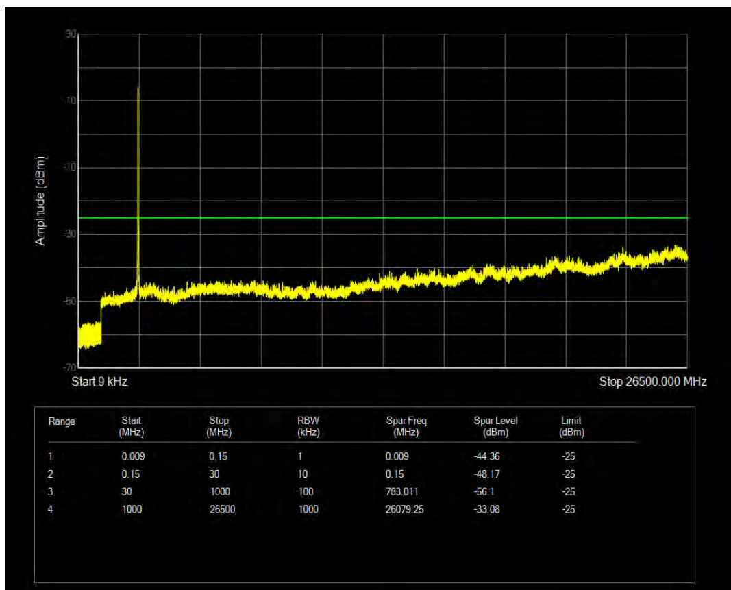
Band41 QPSK BW=20MHz Channel=41340 RB Size=1 Position=#0
