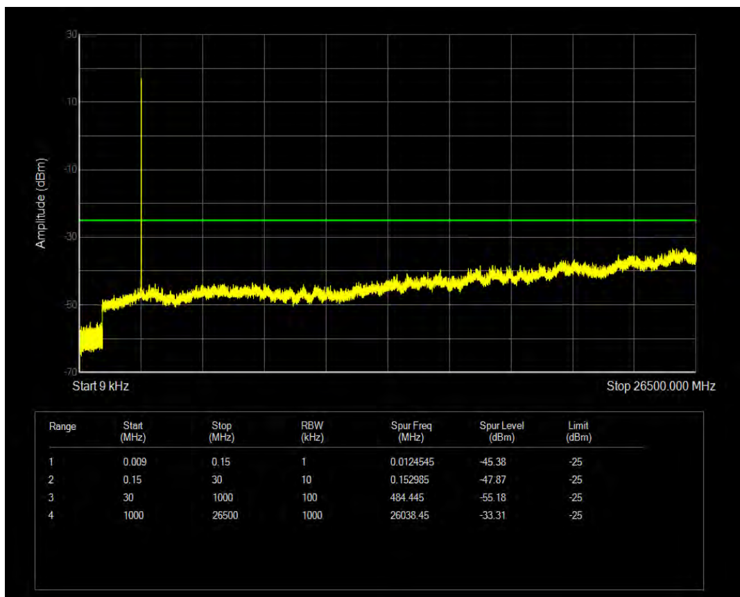
Band41 16QAM BW=5MHz Channel=40740 RB Size=1 Position=#0
