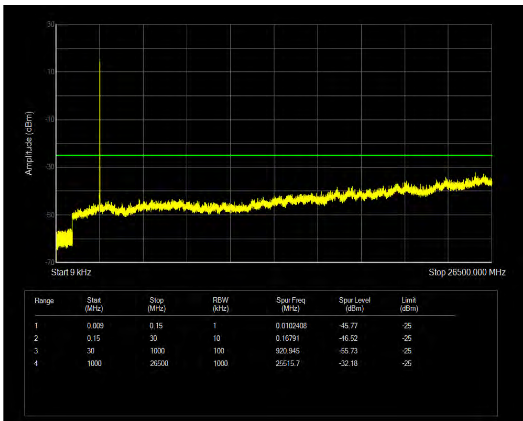
Band41 16QAM BW=15MHz Channel=40115 RB Size=1 Position=#0
