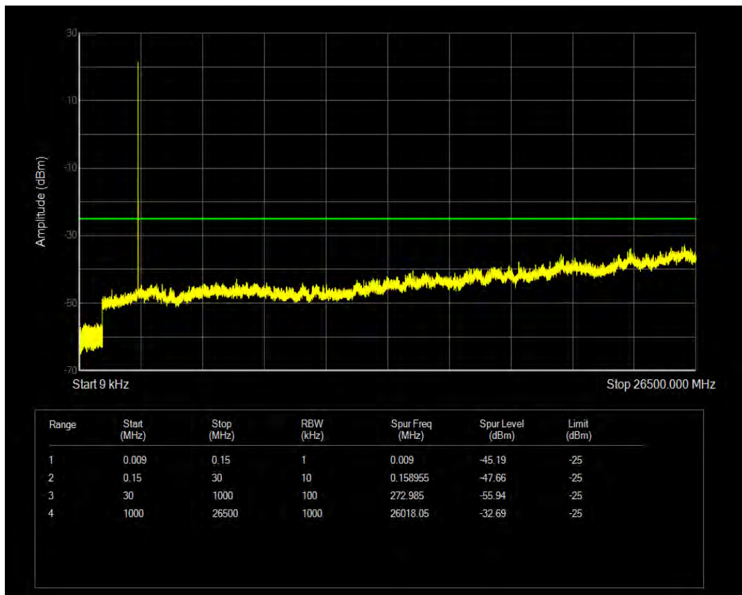
Band41 16QAM BW=5MHz Channel=40065 RB Size=25 Position=#0
