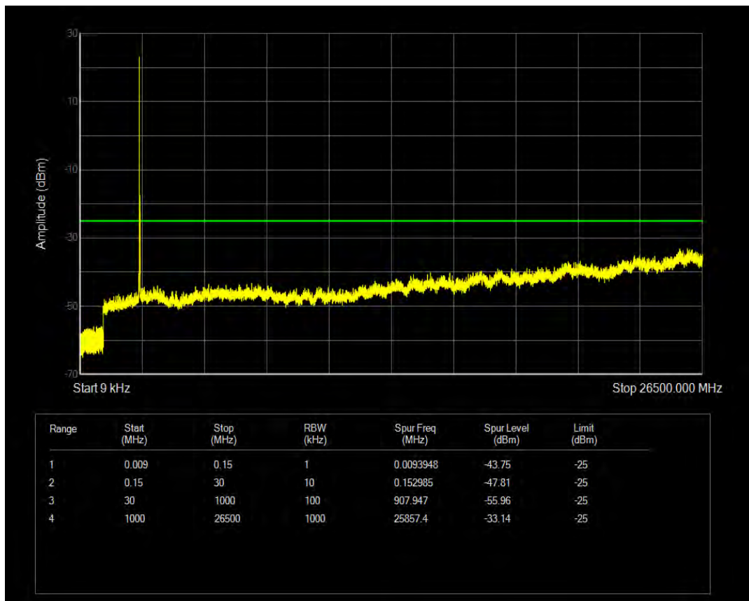
Band41 QPSK BW=15MHz Channel=41365 RB Size=75 Position=#0
