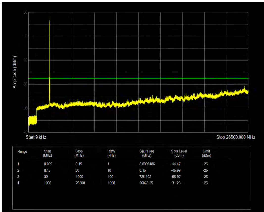
Band41 16QAM BW=15MHz Channel=41365 RB Size=75 Position=#0
