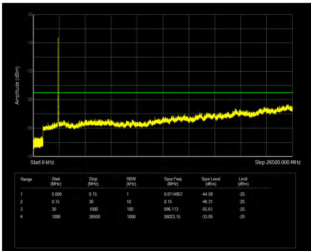
Band41 16QAM BW=20MHz Channel=40740 RB Size=1 Position=#0
