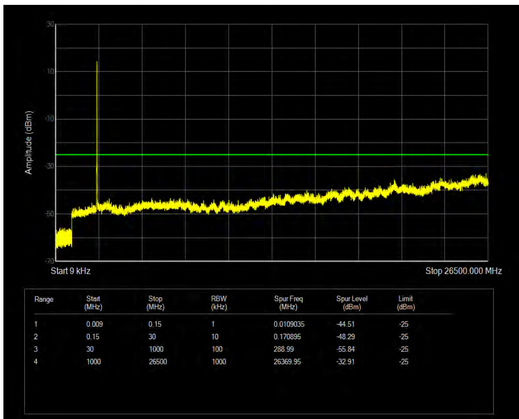
Band41 16QAM BW=15MHz Channel=40740 RB Size=1 Position=#0
