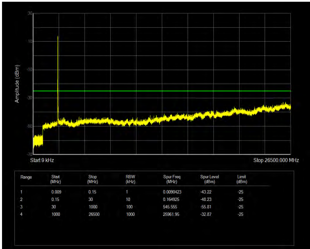
Band41 QPSK BW=20MHz Channel=40740 RB Size=1 Position=#0
