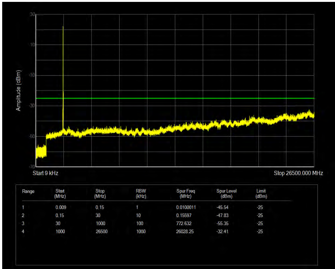
Band41 16QAM BW=5MHz Channel=40065 RB Size=1 Position=#0
