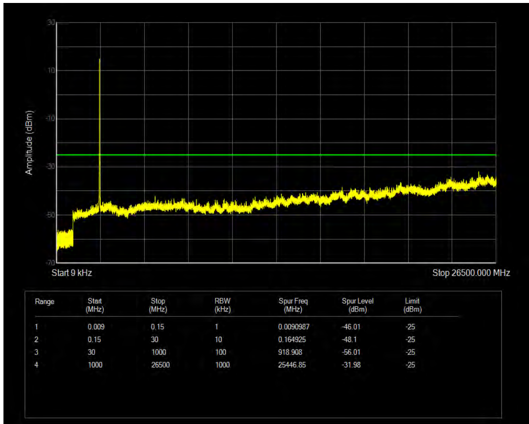
Band41 QPSK BW=15MHz Channel=41365 RB Size=1 Position=#0
