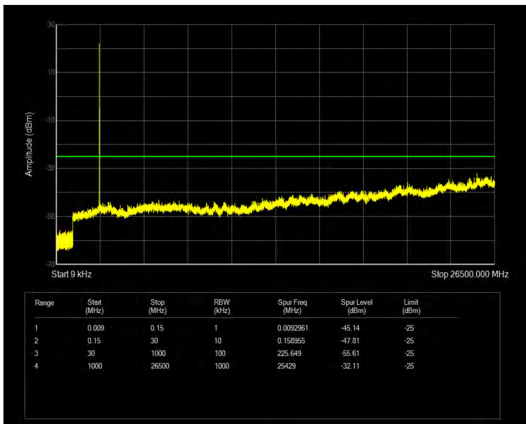
Band41 16QAM BW=5MHz Channel=40740 RB Size=25 Position=#0
