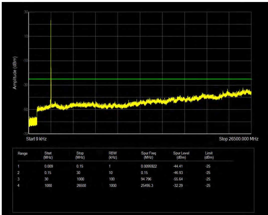
Band41 16QAM BW=20MHz Channel=41340 RB Size=100 Position=#0
