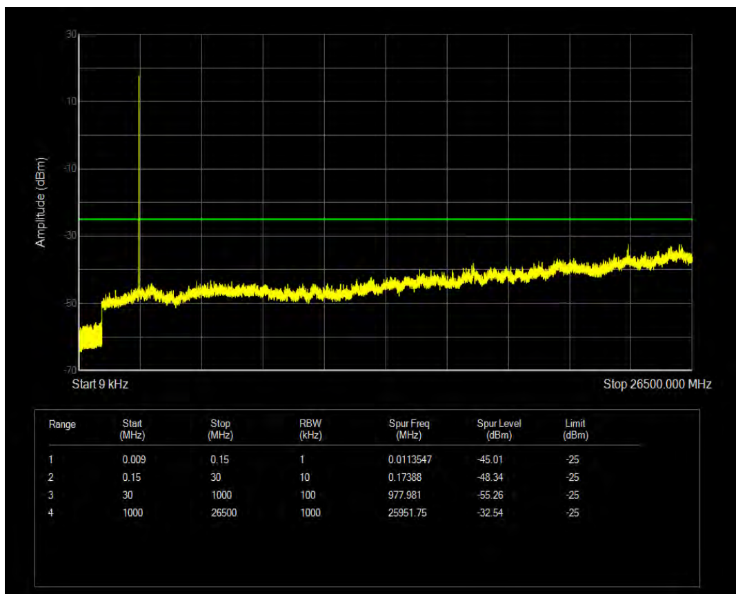
Band41 16QAM BW=20MHz Channel=40740 RB Size=100 Position=#0
