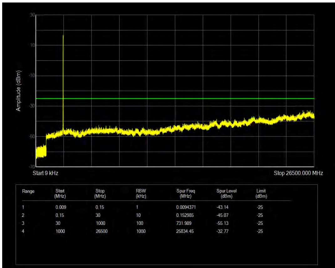
Band41 16QAM BW=10MHz Channel=40090 RB Size=1 Position=#0
