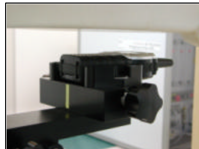
Figure 11. Mouth Face SAR Test Setup
