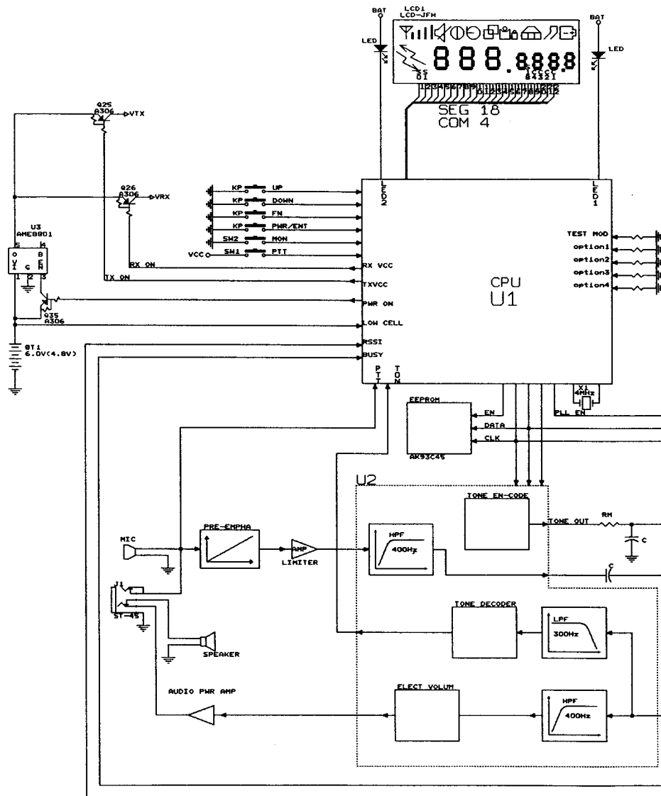
JDF14H BLOCK DIAGRAM
