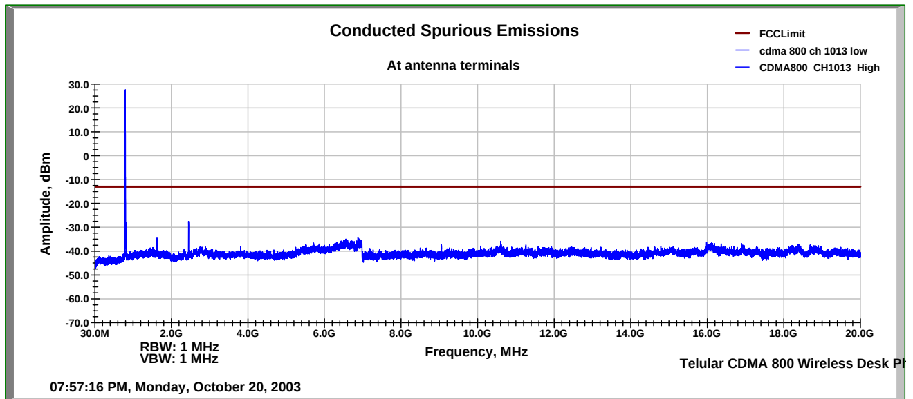
Figure 7-3: Out of band emissions at antenna terminals – CDMA 800 Channel 1013
