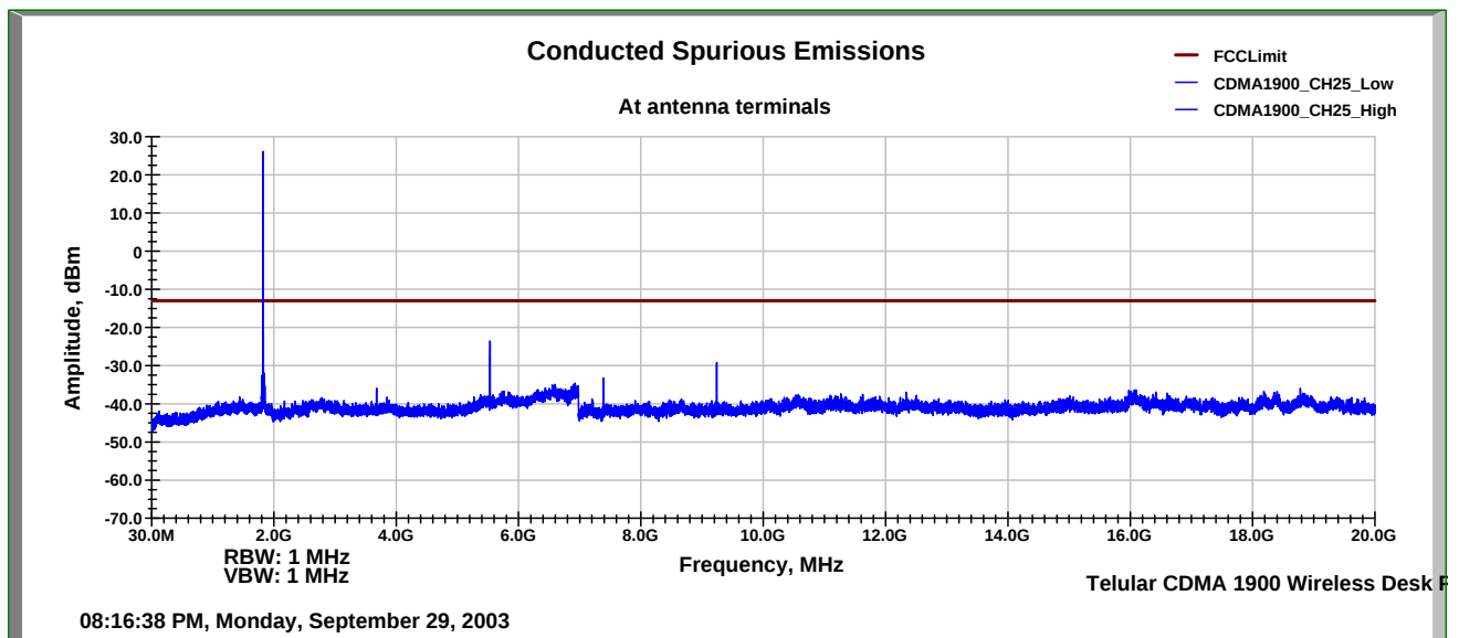
Figure 7-4: Out of band emissions at antenna terminals – CDMA1900 Channel 25
